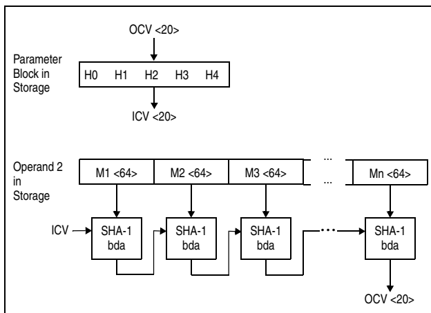
Figure 7-195. KIMD-SHA-1
