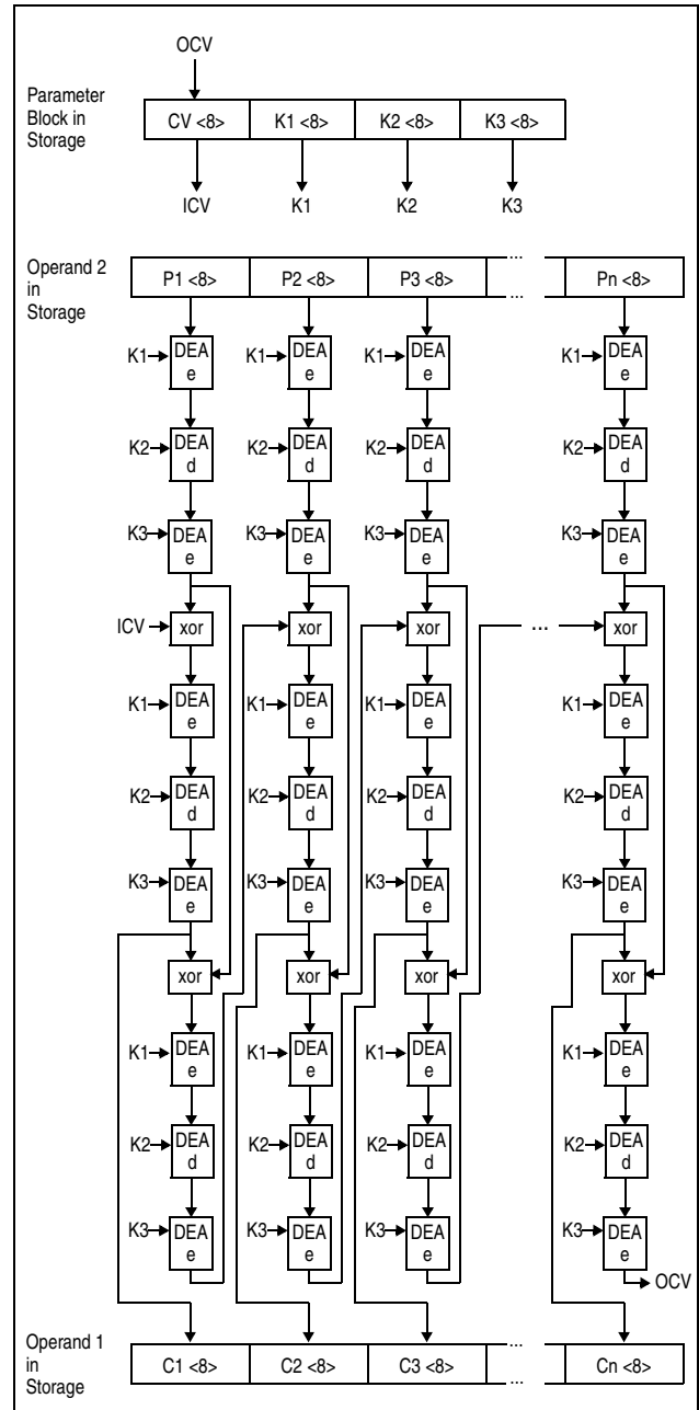
Figure 7-73. KMC-PRNG
