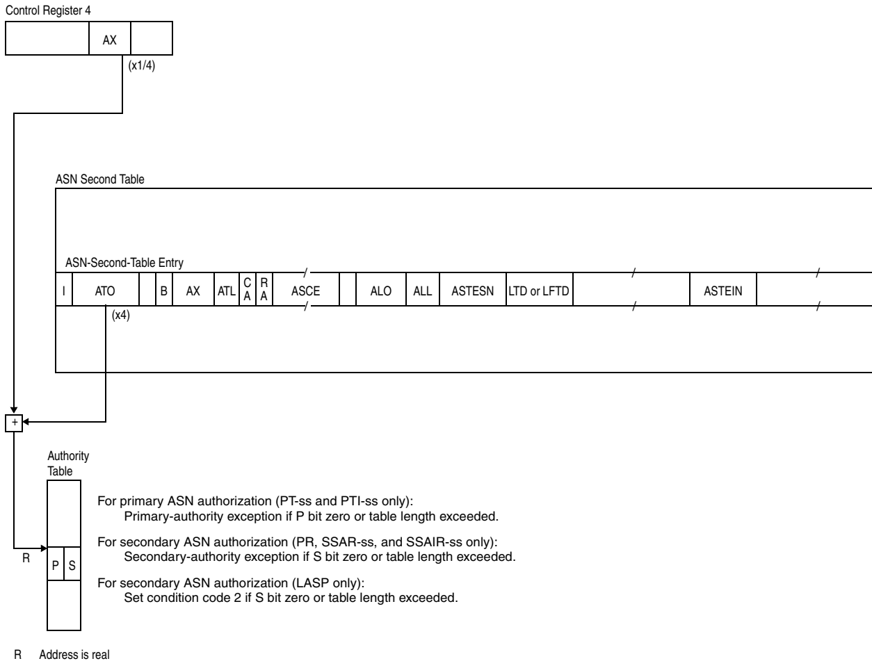
Figure 3-10. ASN Authorization
