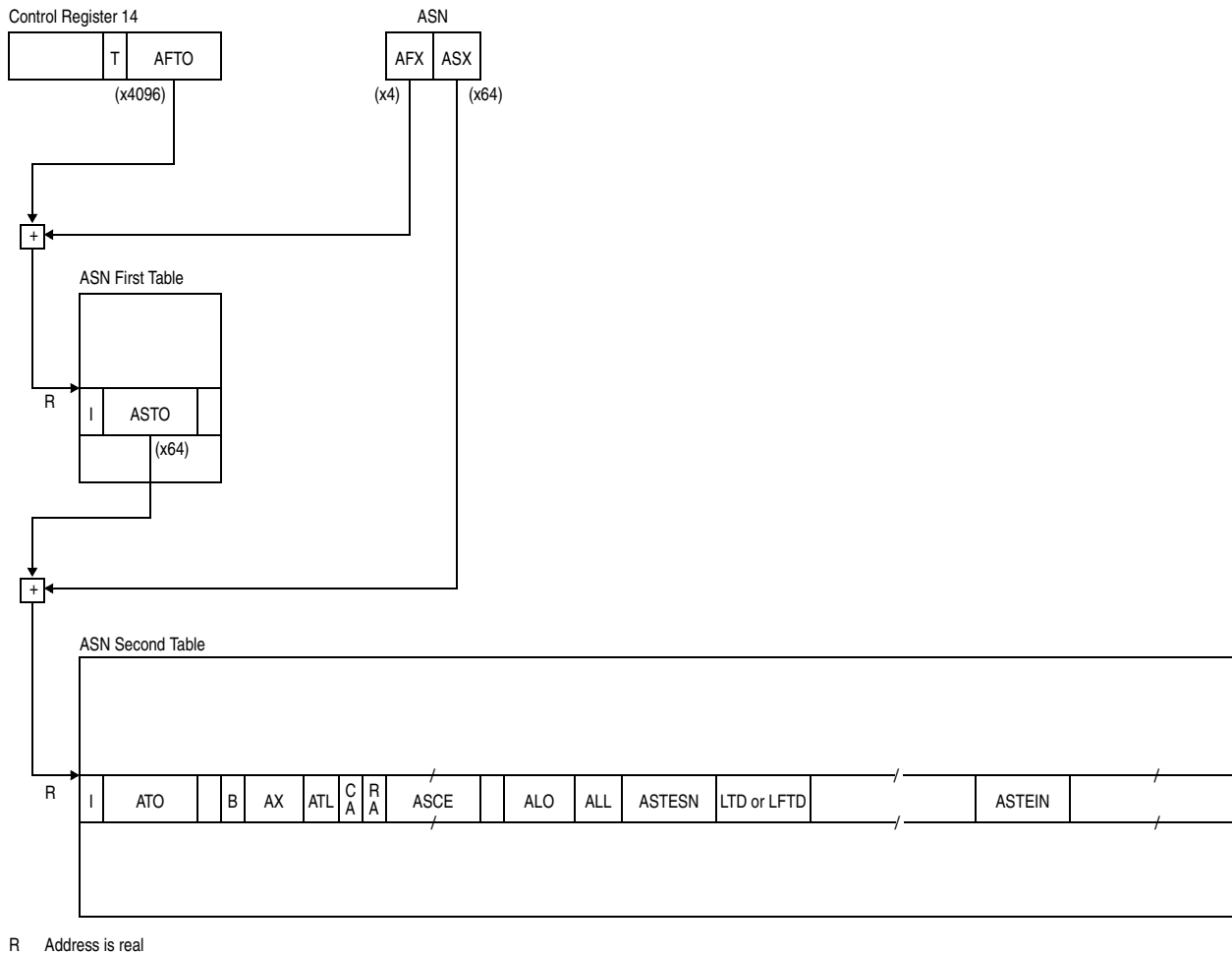
Figure 3-9. ASN Translation
