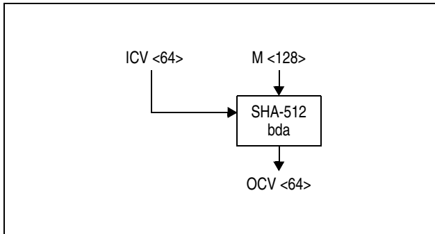
Figure 7-191. Symbol for SHA-512 Block Digest Algorithm
