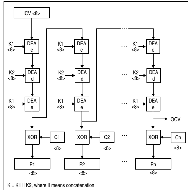
Figure 7-156. KMO-TDEA-128 Decipher Operation
