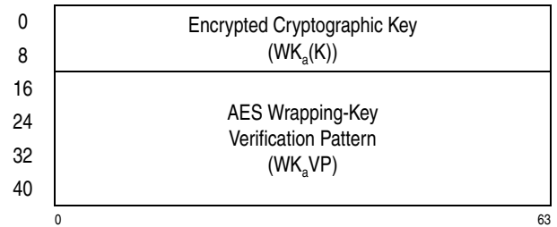
Figure 7-129. Parameter Block for KMCTR-Encrypted-AES-128
