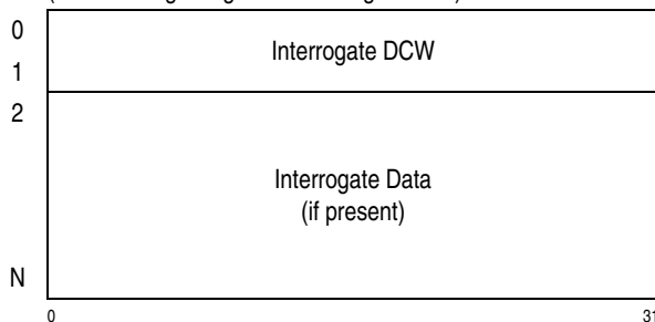
Figure 15-18. Interrogate Transport-Command Area (TCA)
