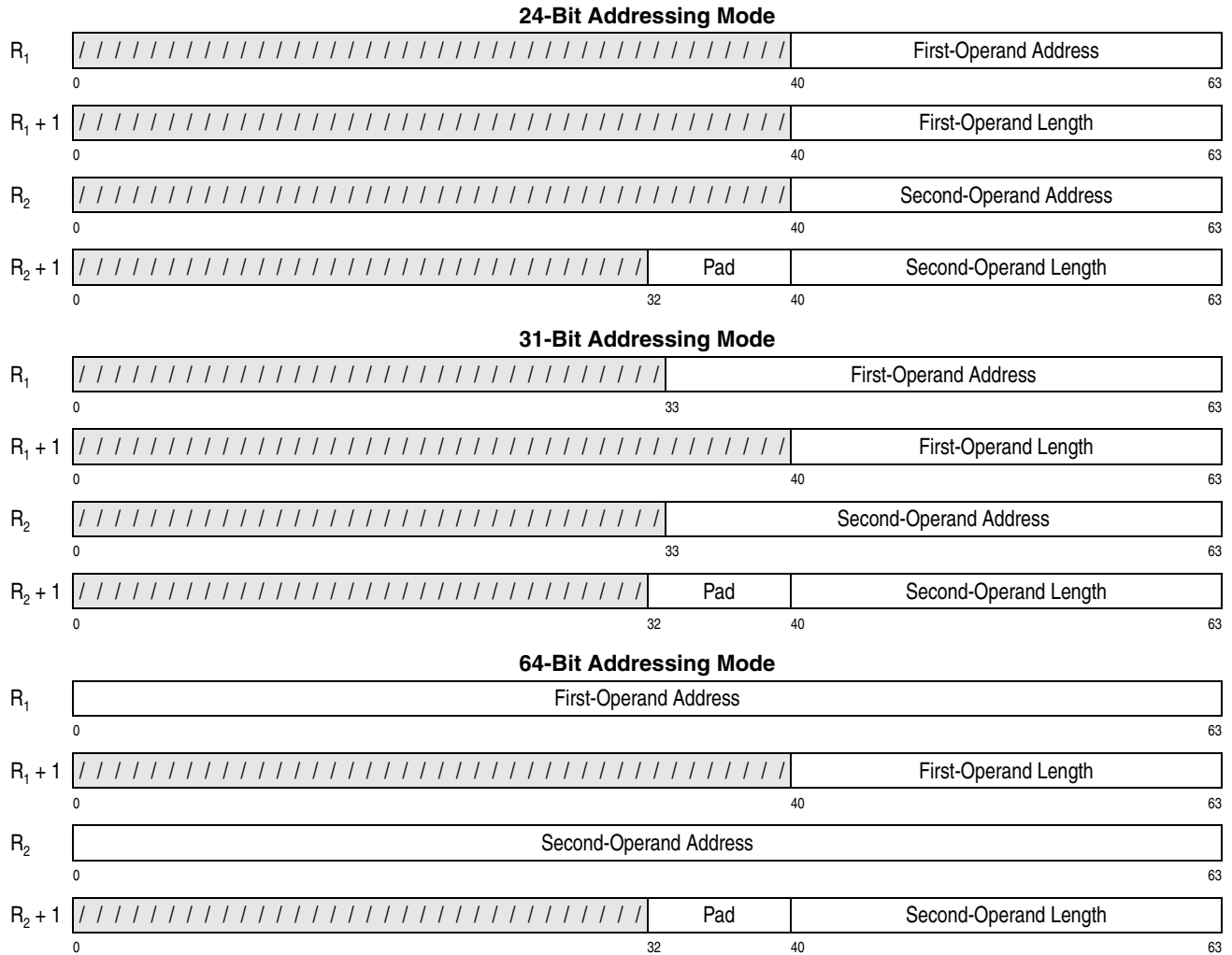
Figure 7-179. Register Contents for COMPARE LOGICAL LONG
