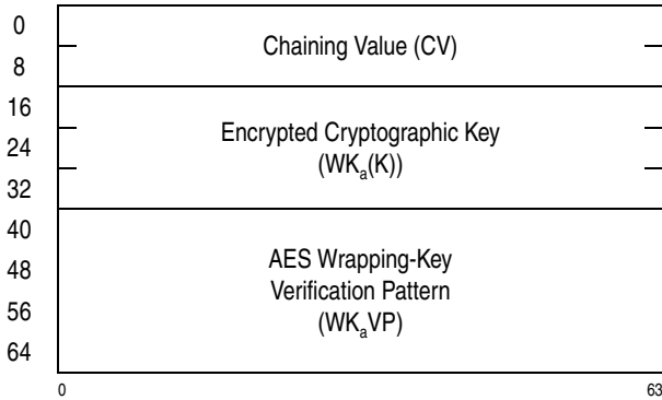
Figure 7-166. Parameter Block for KMO-Encrypted-AES-192
