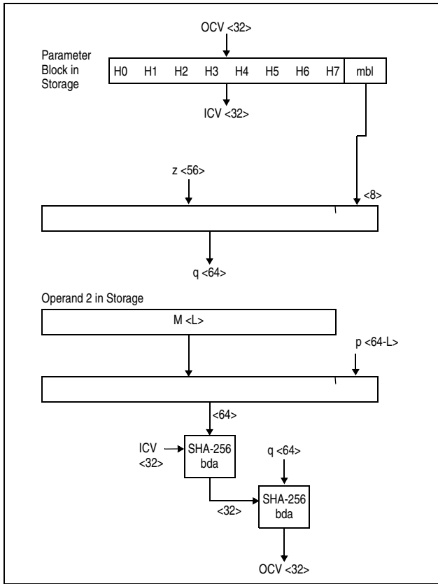
Figure 7-212. KLMD-SHA-256 Partial-Block Case 2 ( 56 \leq L \leq 63 )
