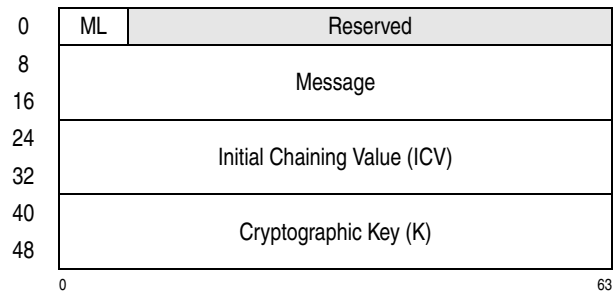
Figure 7-275. Parameter Block for PCC-Compute-Last-Block-CMAC-Using-AES-128
