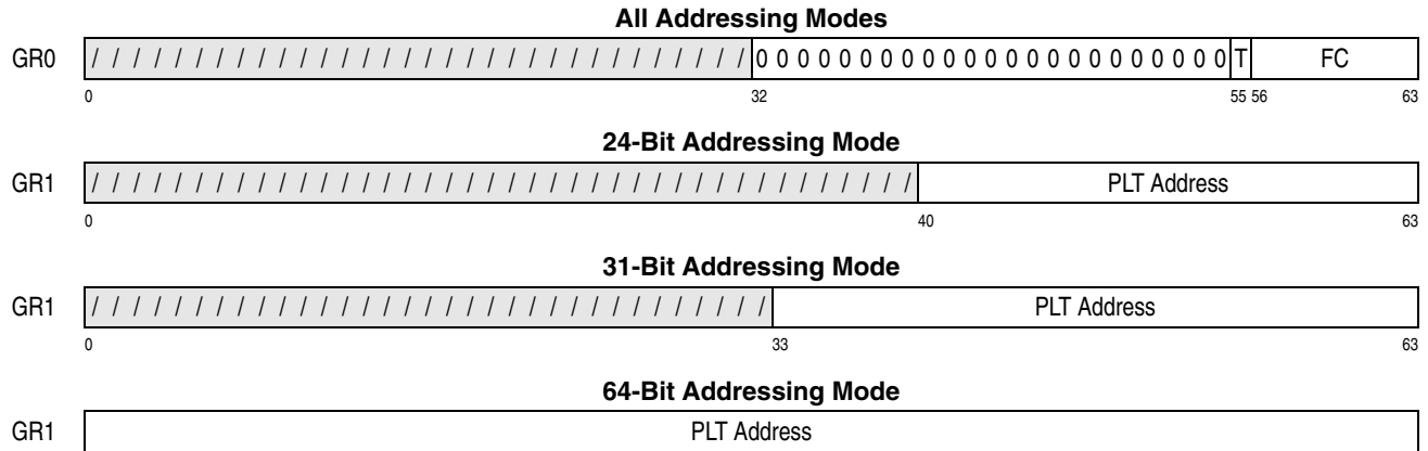
Figure 7-292. General Register Assignment for PLO
