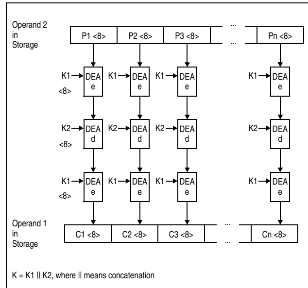
Figure 7-21. KM-TDEA Encipher Operation Using 128-Bit Key
