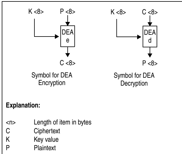
Figure 7-318. Symbols for DEA Encryption and Decryption
