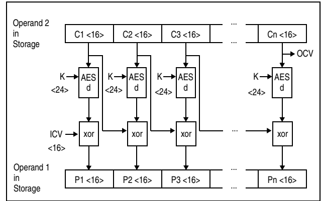
Figure 7-67. KMC AES Decipher Operation Using 192-Bit Key
