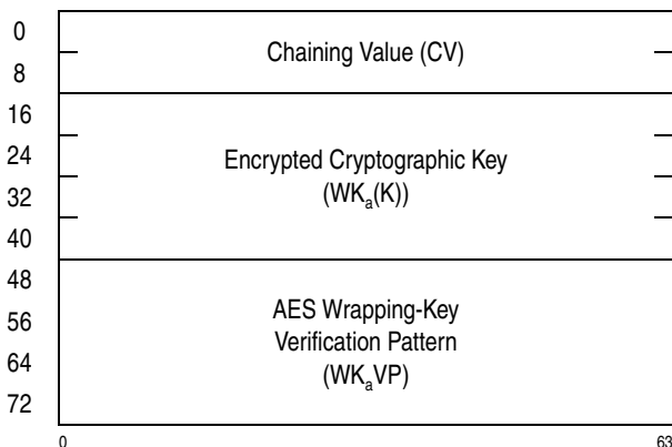
Figure 7-104. Parameter Block for KMF-AES-256
