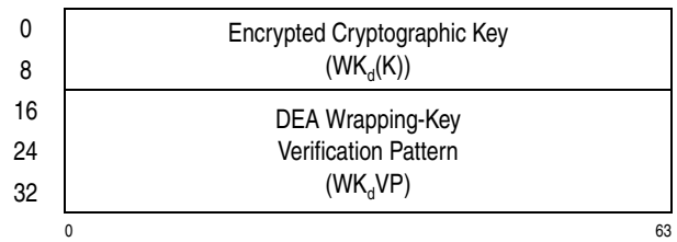
Figure 7-121. Parameter Block for KMCTR Encrypted-TDEA-128
