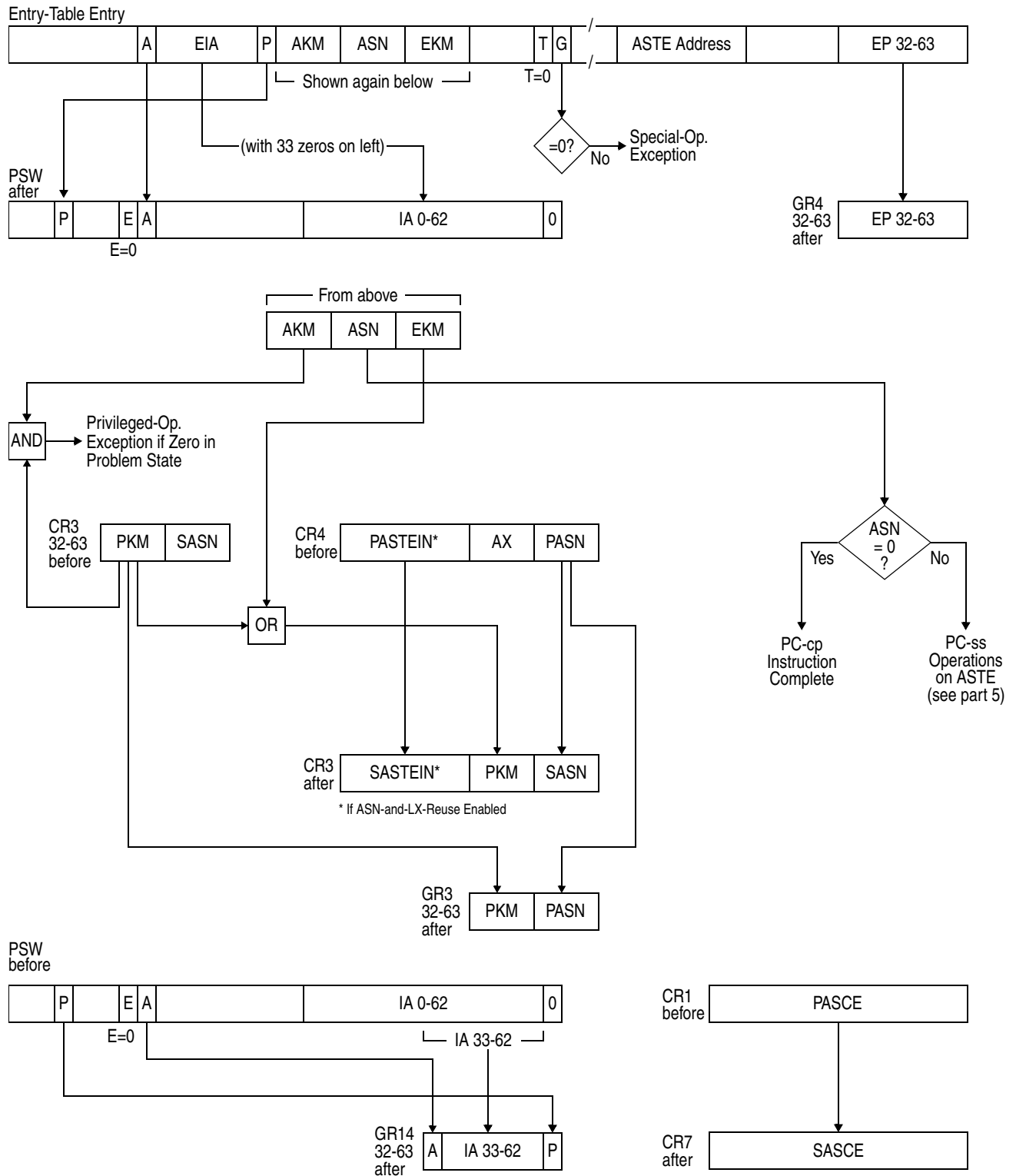
Figure 10-63. Execution of PROGRAM CALL (Part 1 of 5).
