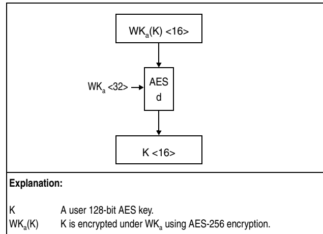
Figure 7-323. Decryption of 128-Bit AES Key Using WK_a
