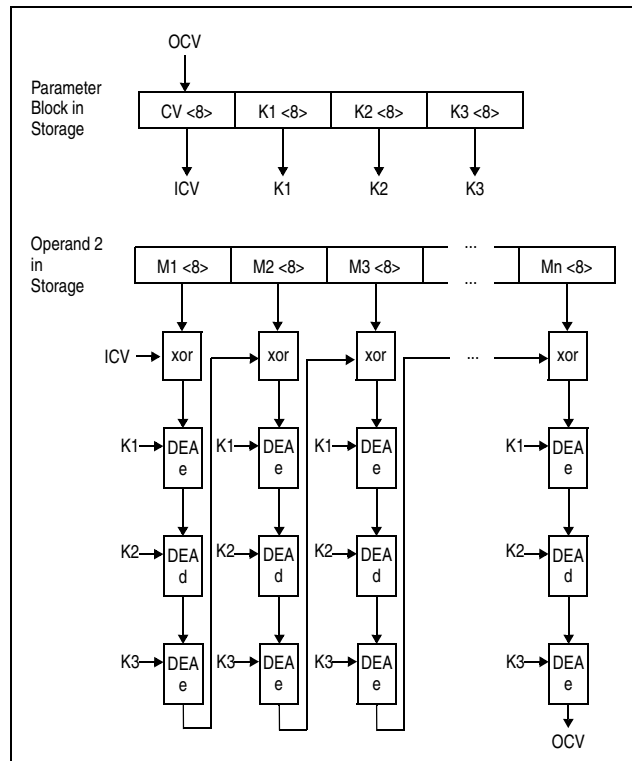
Figure 7-235. MAC Computation Using 192-bit TDEA Key
