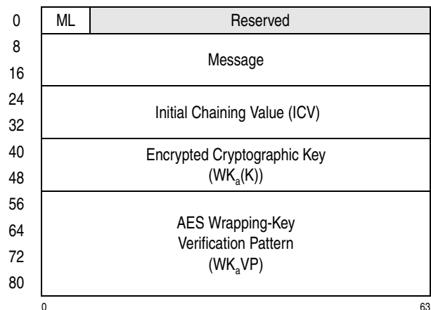
Figure 7-276. Parameter Block for PCC-Compute-Last-Block-CMAC-Using-Encrypted-AES-128
