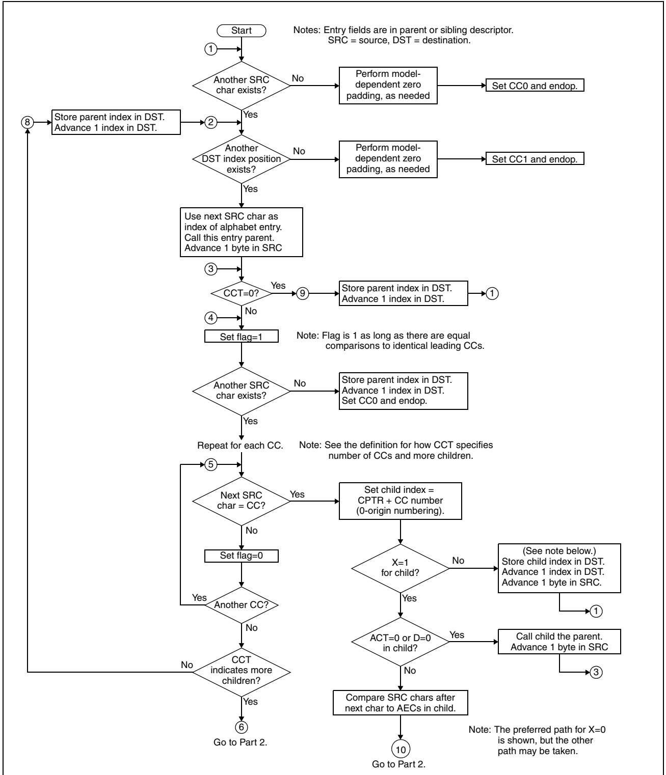
Figure 7-184. Compression Process (Part 1 of 2)
