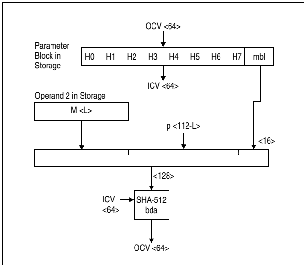
Figure 7-216. KLMD-SHA-512 Partial-Block Case 1 ( 1 \leq L \leq 111 )
