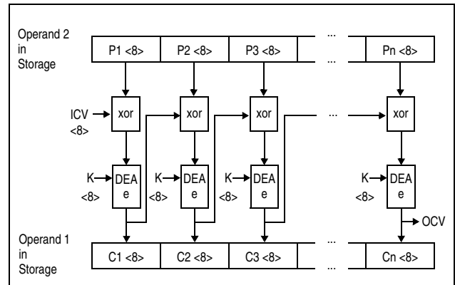
Figure 7-50. KMC DEA Encipher Operation Using 64-Bit Key
