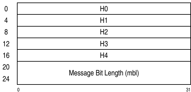
Figure 7-203. Parameter Block for KLMD-SHA-1
