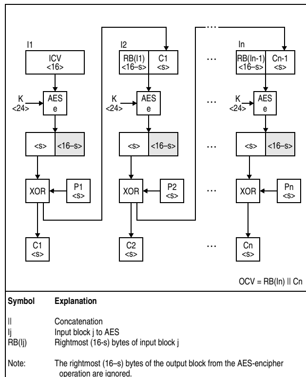
Figure 7-101. KMF-AES-192 Encipher Operation
