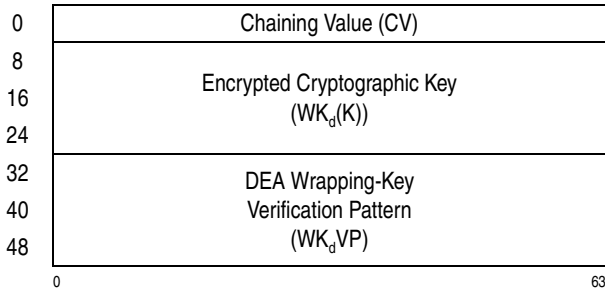
Figure 7-57. Parameter Block for KMC-Encrypted-TDEA-192
