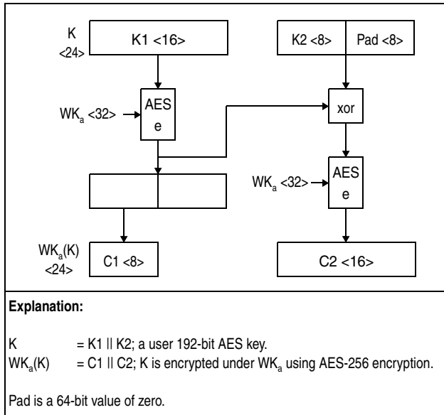
Figure 7-324. Encryption of 192-Bit AES Key Using WK_a
