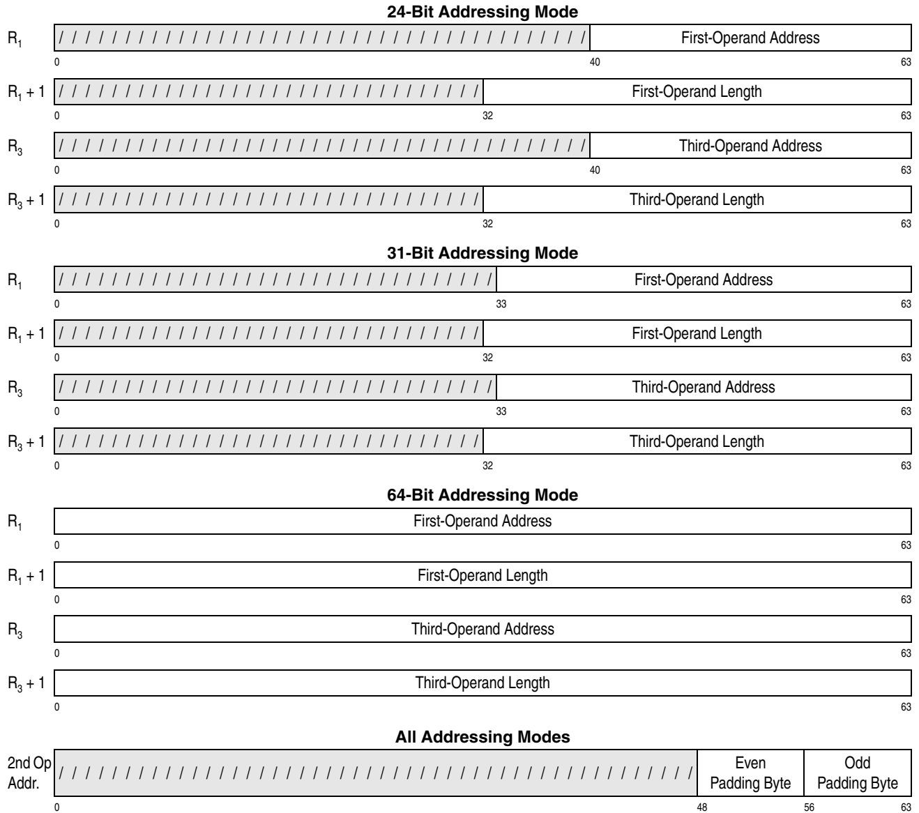
Figure 7-255. Register Contents and Second-Operand Address for MOVE LONG UNICODE
