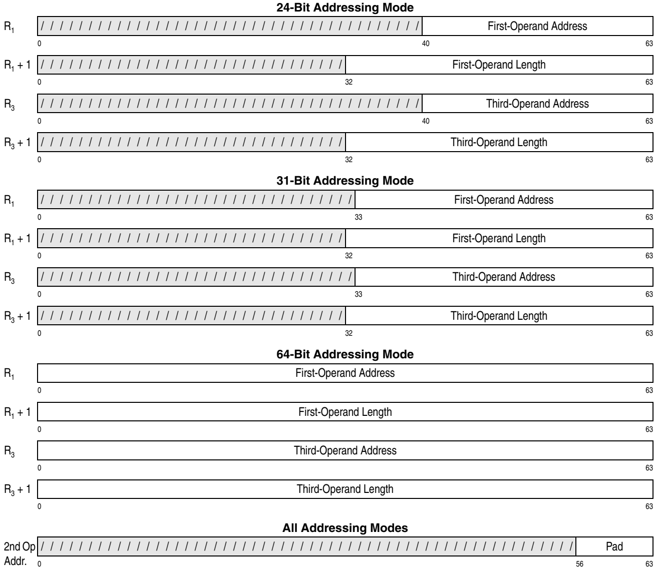
Figure 7-180. Register Contents and Second-Operand Address for COMPARE LOGICAL LONG EXTENDED
