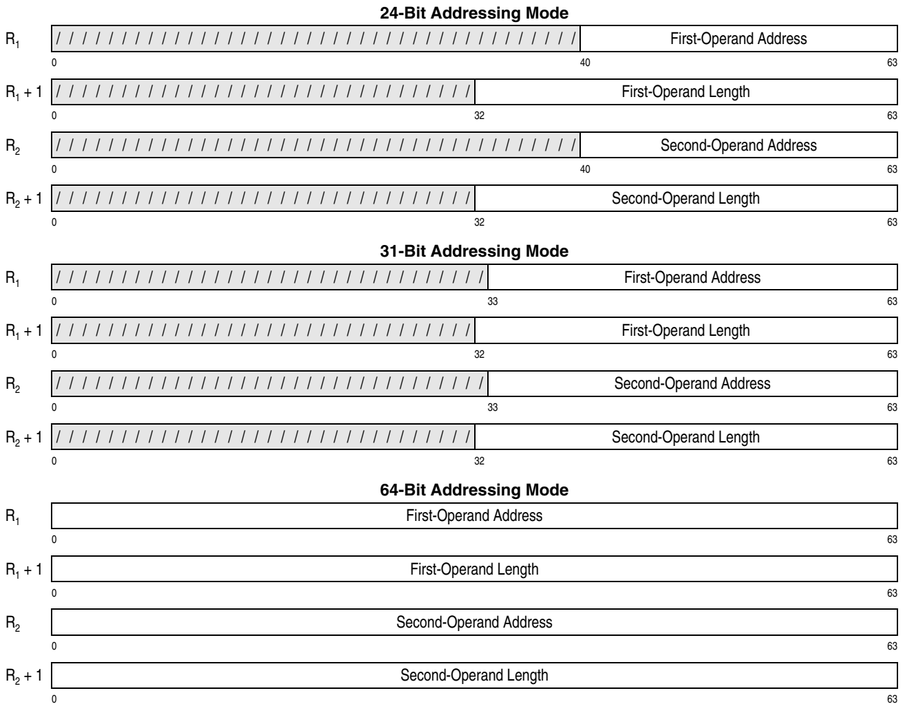
Figure 7-249. Register Contents for CONVERT UTF-32 TO UTF-8
