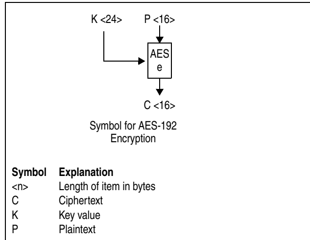
Figure 7-113. Symbols for AES-192 Encryption
