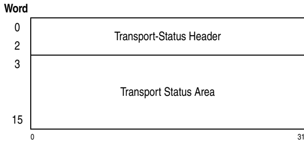
Figure 15-20. Transport-Status Block
