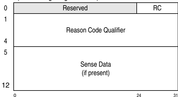
Figure 15-23. Device-Detected-Program-Check Transport-Status Area (TSA)
