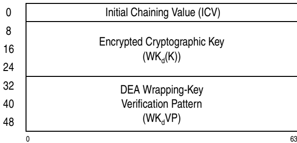
Figure 7-234. Parameter Block for KMAC-Encrypted-TDEA-192
