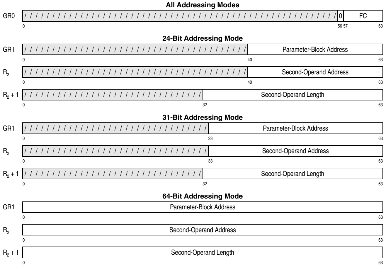
Figure 7-220. General Register Assignment for KMAC
