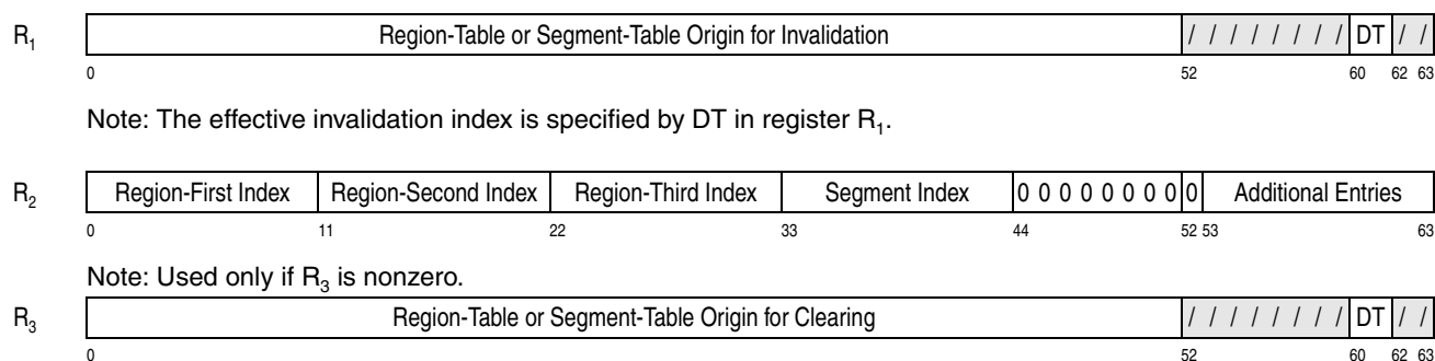
Figure 10-15. Register Contents for INVALIDATE DAT TABLE ENTRY Invalidation-and-Clearing Operation (Bit 52 of GR R 2 Is Zero)
