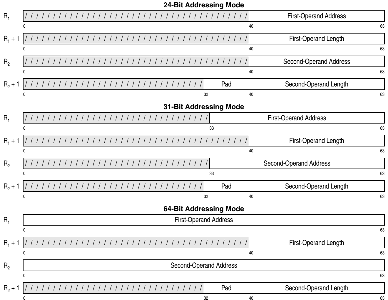
Figure 7-253. Register Contents for MOVE LONG
