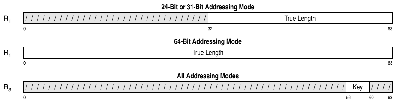
Figure 10-33. Register Contents of MOVE WITH KEY
