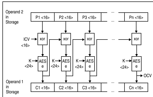
Figure 7-66. KMC AES Encipher Operation Using 192-Bit Key
