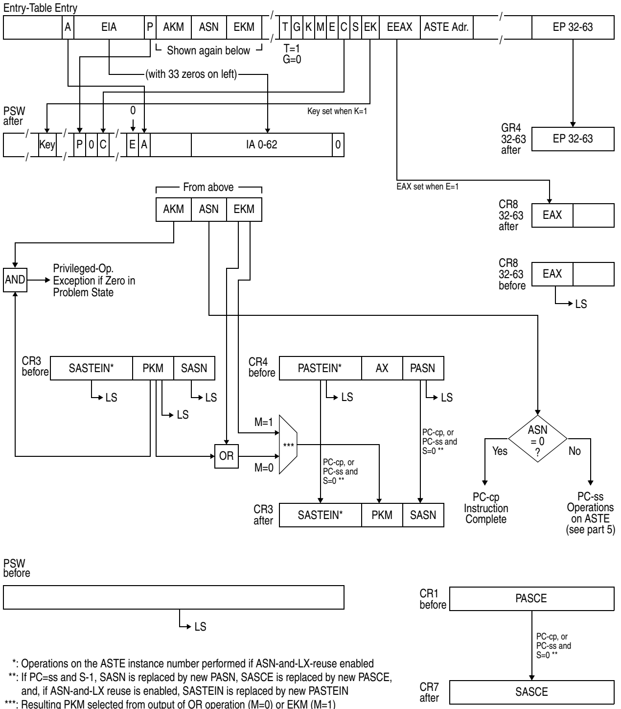
Figure 10-63. Execution of PROGRAM CALL (Part 4 of 5).
