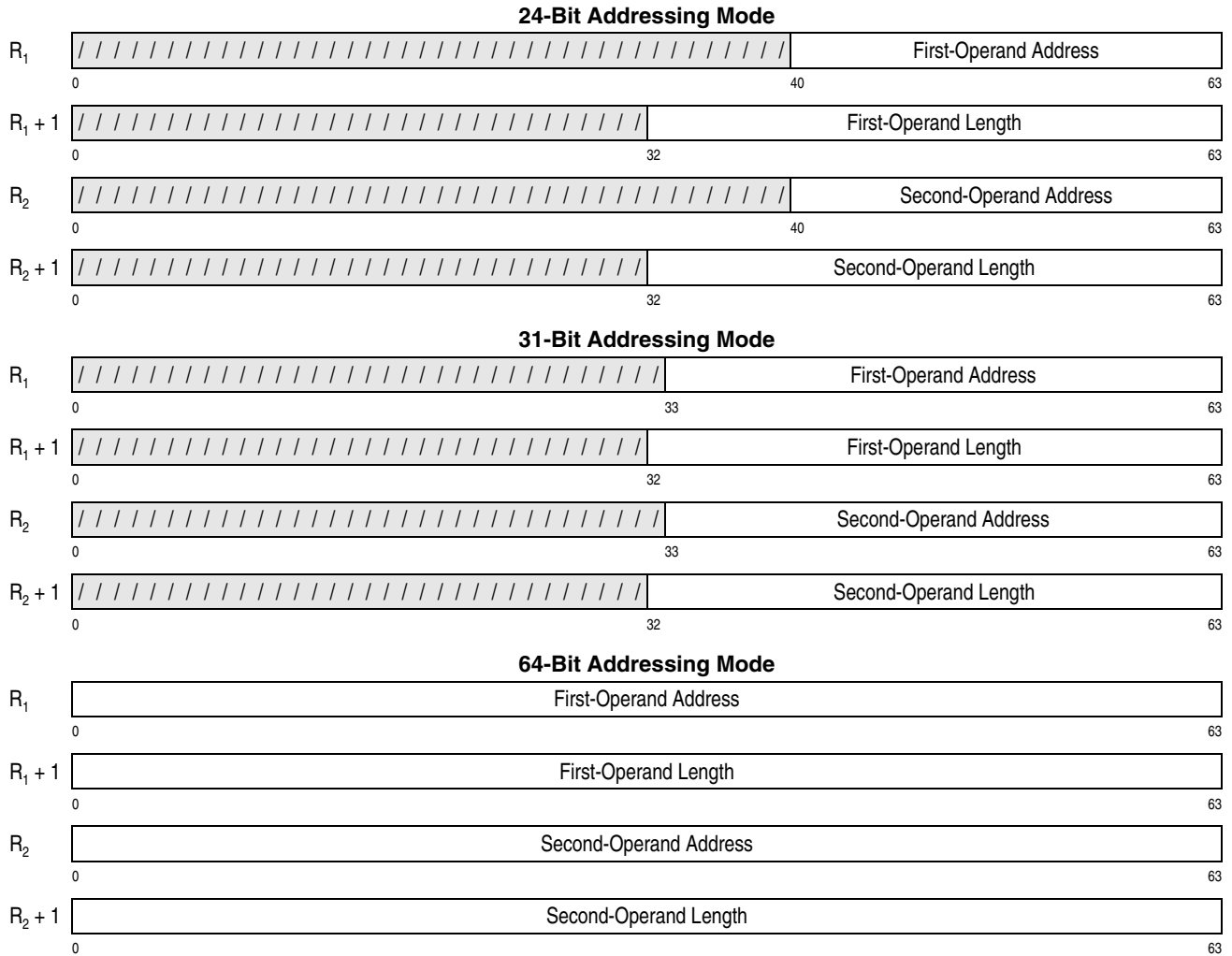
Figure 7-247. Register Contents for CONVERT UTF-16 TO UTF-8
