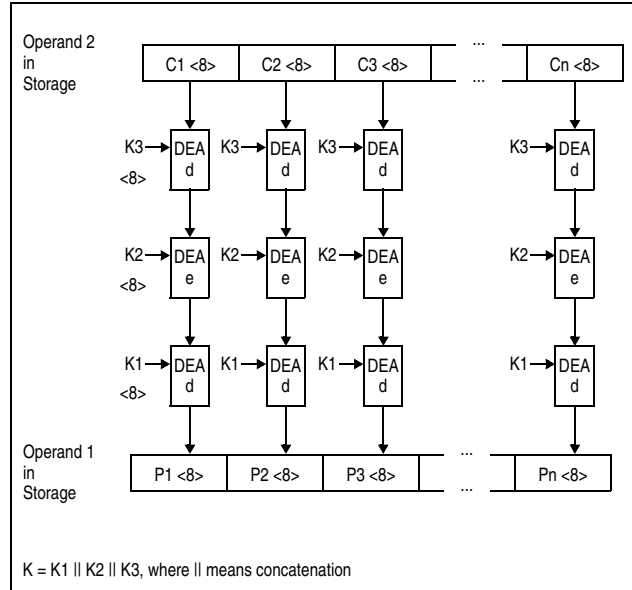
Figure 7-26. KM TDEA Decipher Operation Using 192-Bit Key
