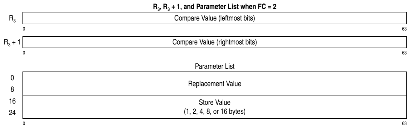
Figure 7-178. Register Contents for COMPARE AND SWAP AND STORE
