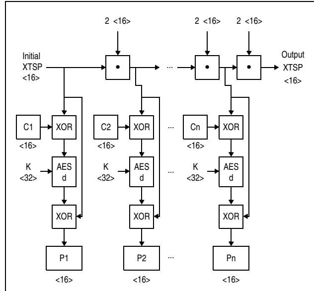
Figure 7-46. XTS-AES-256 Decipher Operation
