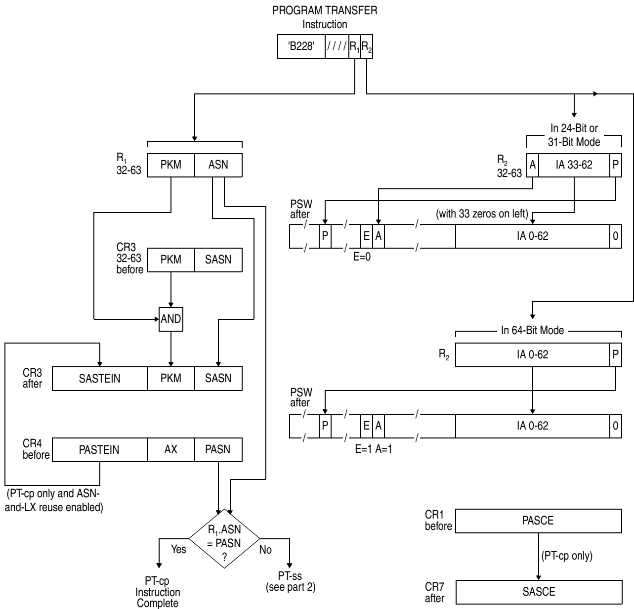
Figure 10-67. Execution of PROGRAM TRANSFER (Part 1 of 2).
