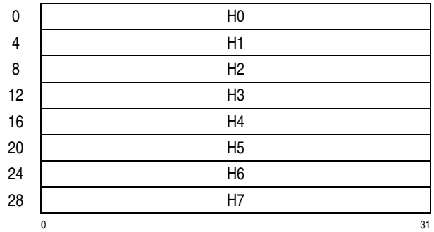
Figure 7-196. Parameter Block for KIMD-SHA-256
