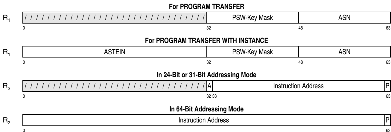
Figure 10-65. Register Contents for PROGRAM TRANSFER (WITH INSTANCE)
