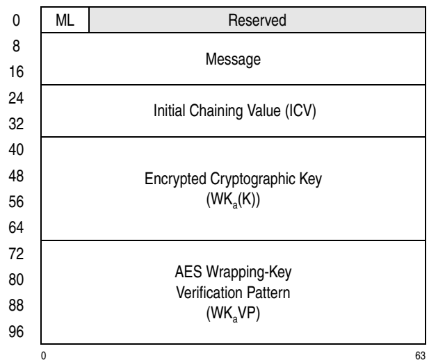
Figure 7-282. Parameter Block for PCC-Compute-Last-Block-CMAC-Using-Encrypted-AES-256
