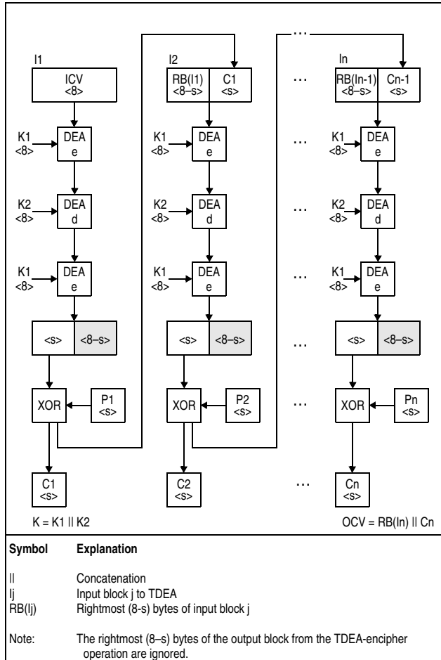
Figure 7-89. KMF-TDEA-128 Encipher Operation
