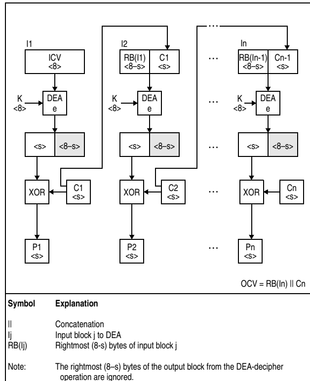
Figure 7-86. KMF-DEA Decipher Operation
