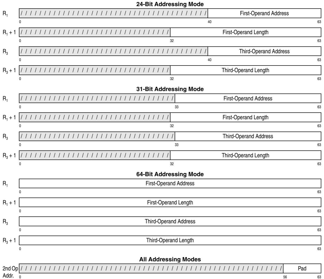
Figure 7-254. Register Contents and Second-Operand Address for MOVE LONG EXTENDED
