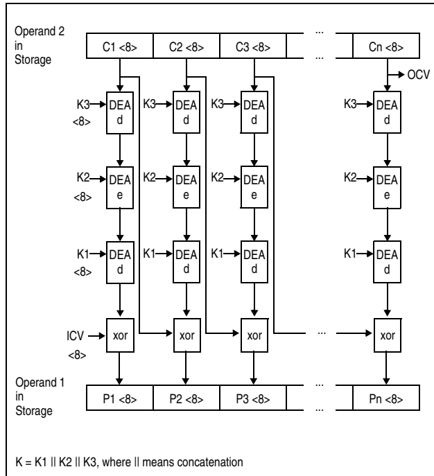
Figure 7-59. KMC TDEA Decipher Operation Using 192-Bit Key
