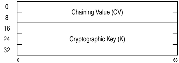
Figure 7-99. Parameter Block for KMF-AES-192
