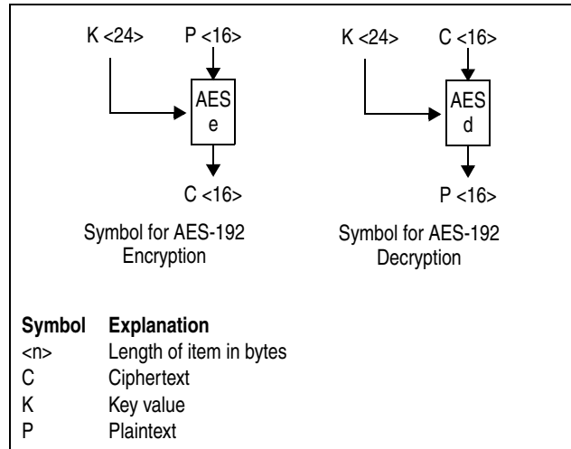
Figure 7-12. Symbols for AES-192 Encryption and Decryption
