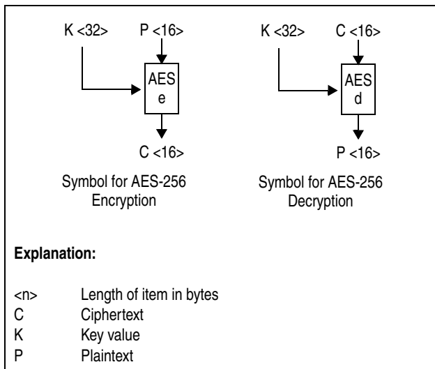
Figure 7-319. Symbols for AES-256 Encryption and Decryption
