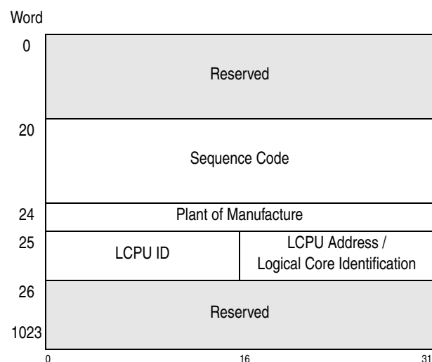
Figure 10-78. Format of the SYSIB 2.2.1
