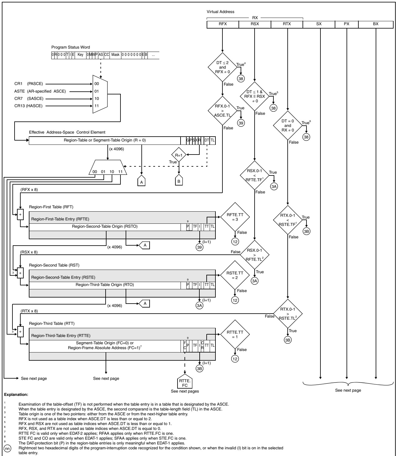
Figure 3-12. Translation Process (Part 1 of 3)
