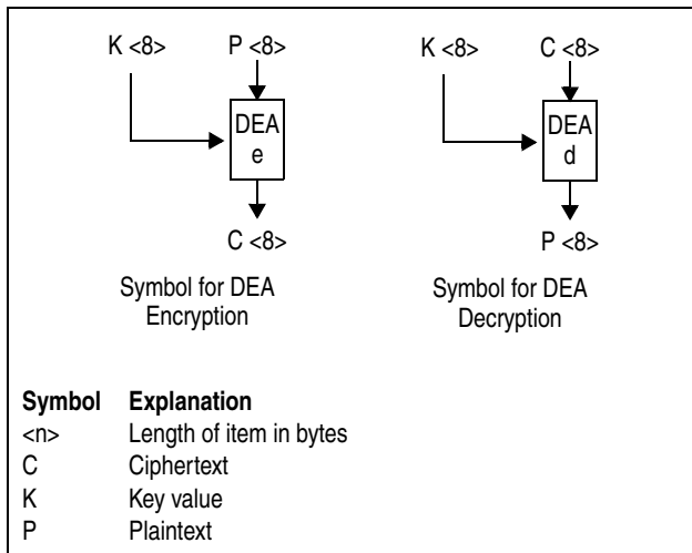
Figure 7-144. Symbols for DEA Encryption and Decryption
