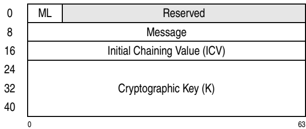
Figure 7-272. Parameter Block for PCC-Compute-Last-Block-CMAC-Using-TDEA-192
