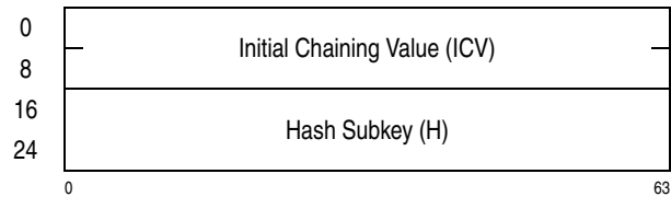
Figure 7-200. Parameter Block for KIMD-GHASH
