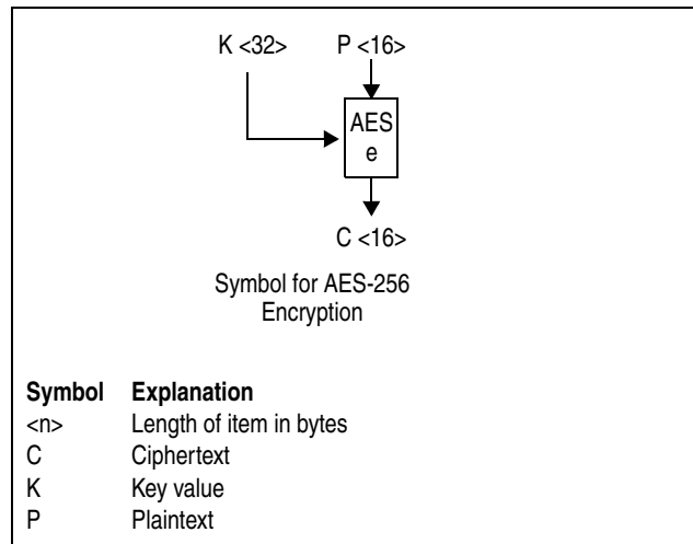
Figure 7-114. Symbols for AES-256 Encryption
