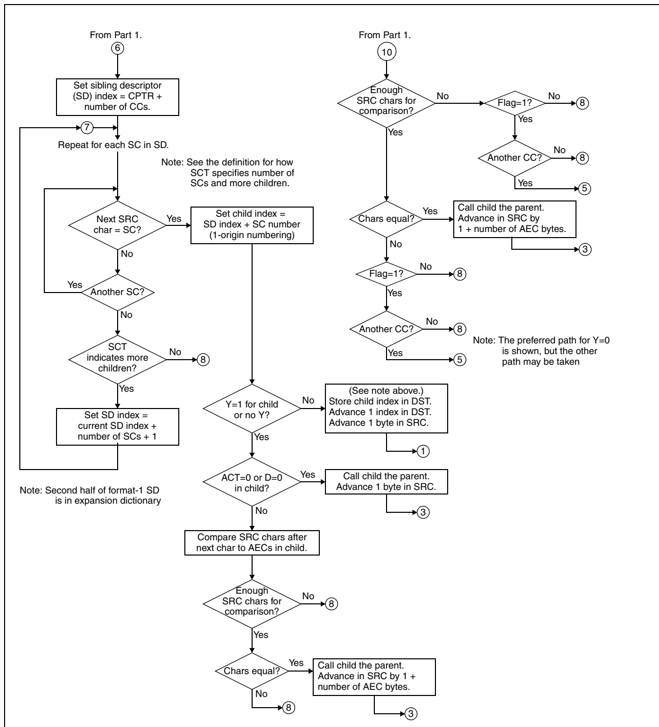
Figure 7-184. Compression Process (Part 2 of 2)
