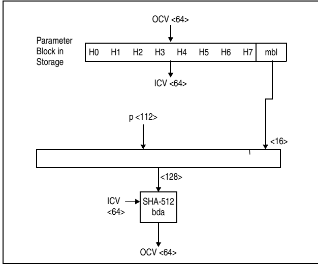
Figure 7-215. KLMD-SHA-512 Empty Block ( L = 0 )
