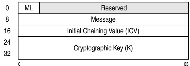
Figure 7-269. Parameter Block for PCC-Compute-Last-Block-CMAC-Using-TDEA-128
