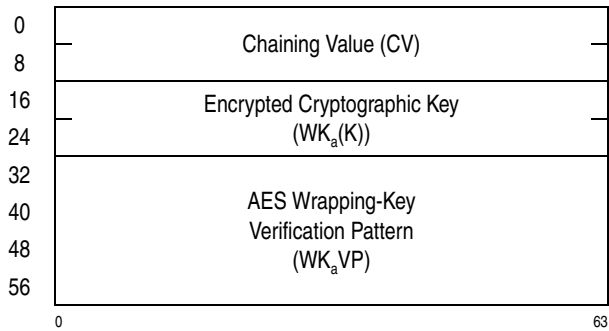
Figure 7-96. Parameter Block for KMF-Encrypted-AES-128
