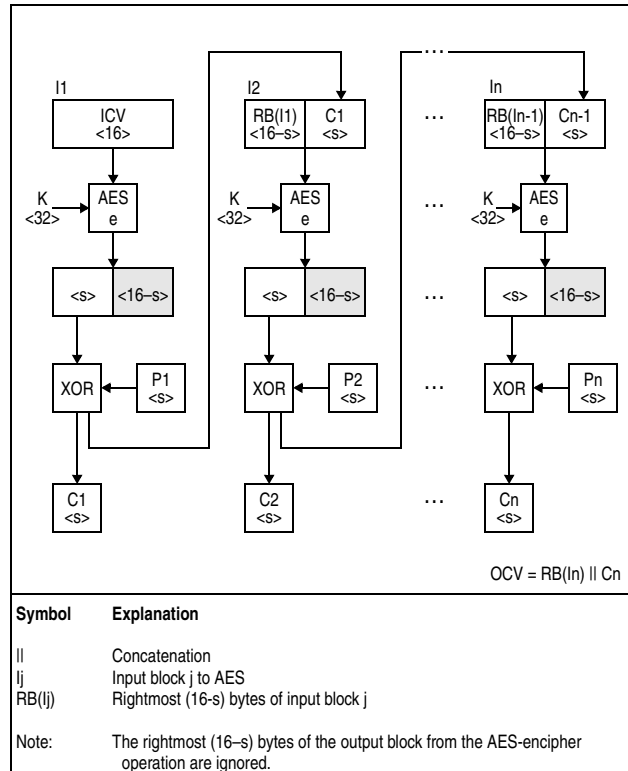
Figure 7-105. KMF-AES-256 Encipher Operation
