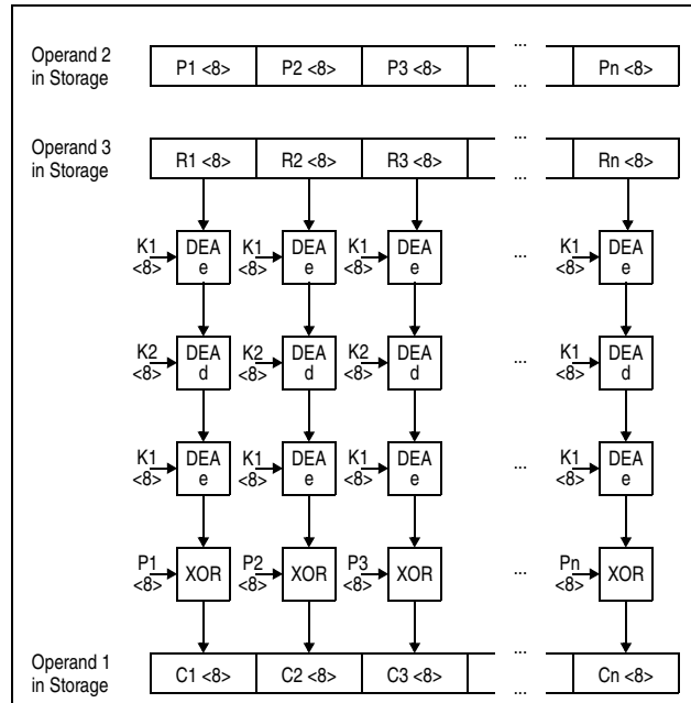
Figure 7-122. KMCTR TDEA Encipher Operation Using 128-Bit Key
