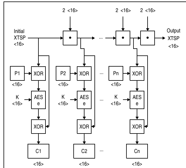
Figure 7-41. KM-XTS-AES-128 Encipher Operation
