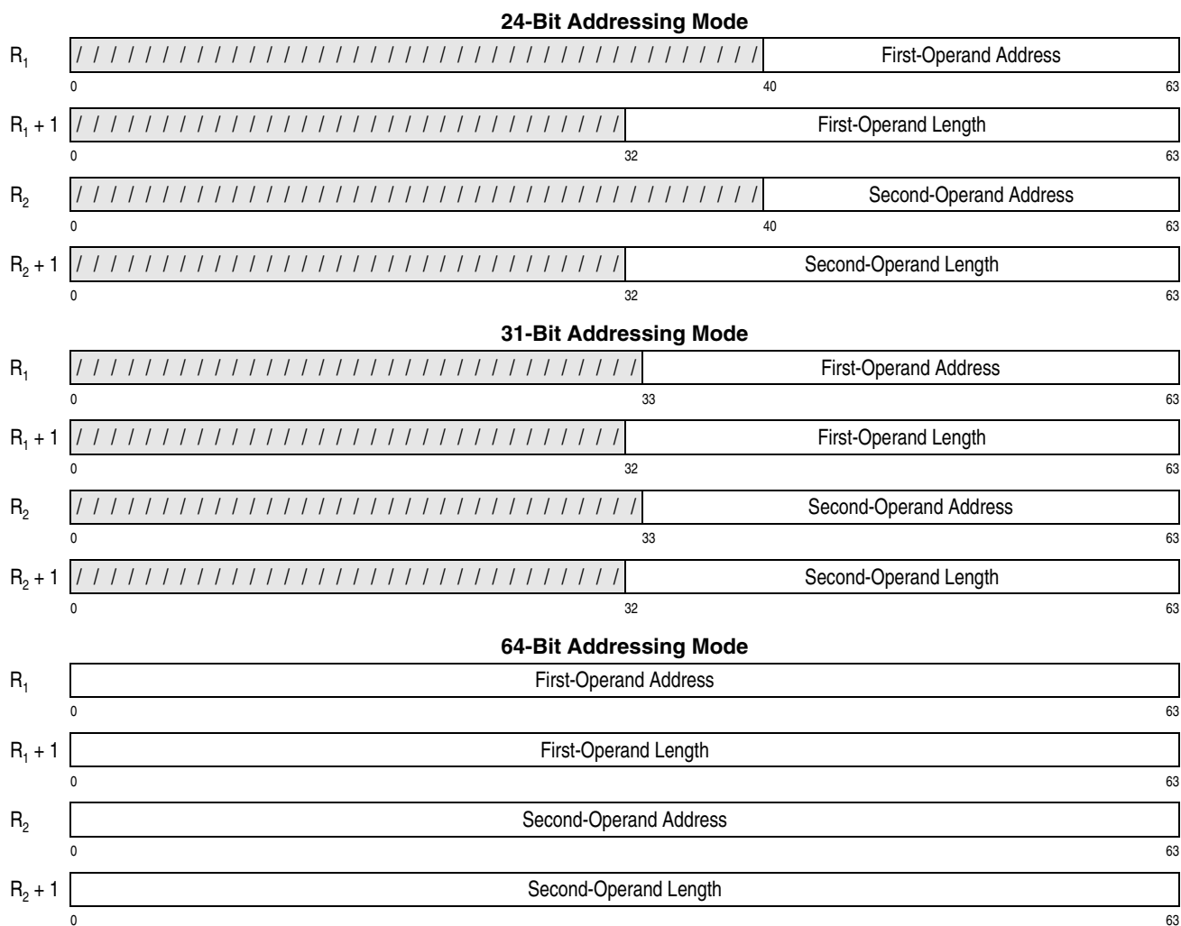
Figure 7-248. Register Contents for CONVERT UTF-32 TO UTF-16
