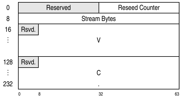
Figure 7-299. Parameter Block for PPNO-SHA-512-DRNG Function
