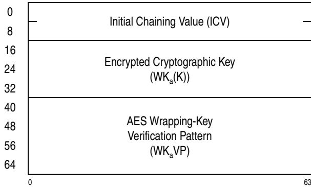
Figure 7-240. Parameter Block for KMAC-Encrypted-AES-192
