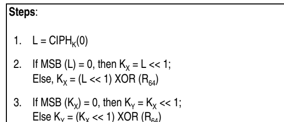
Figure 7-274. Subkey Generation Algorithm
