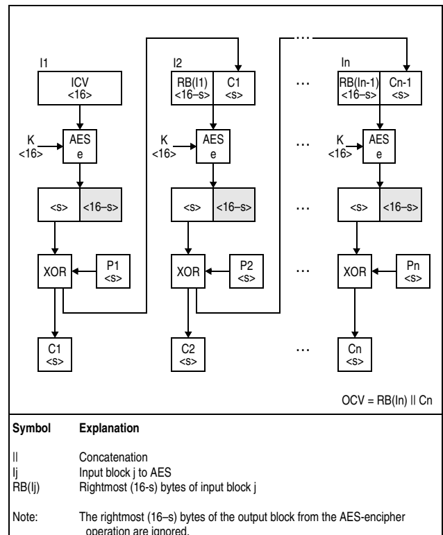
Figure 7-97. KMF-AES-128 Encipher Operation
