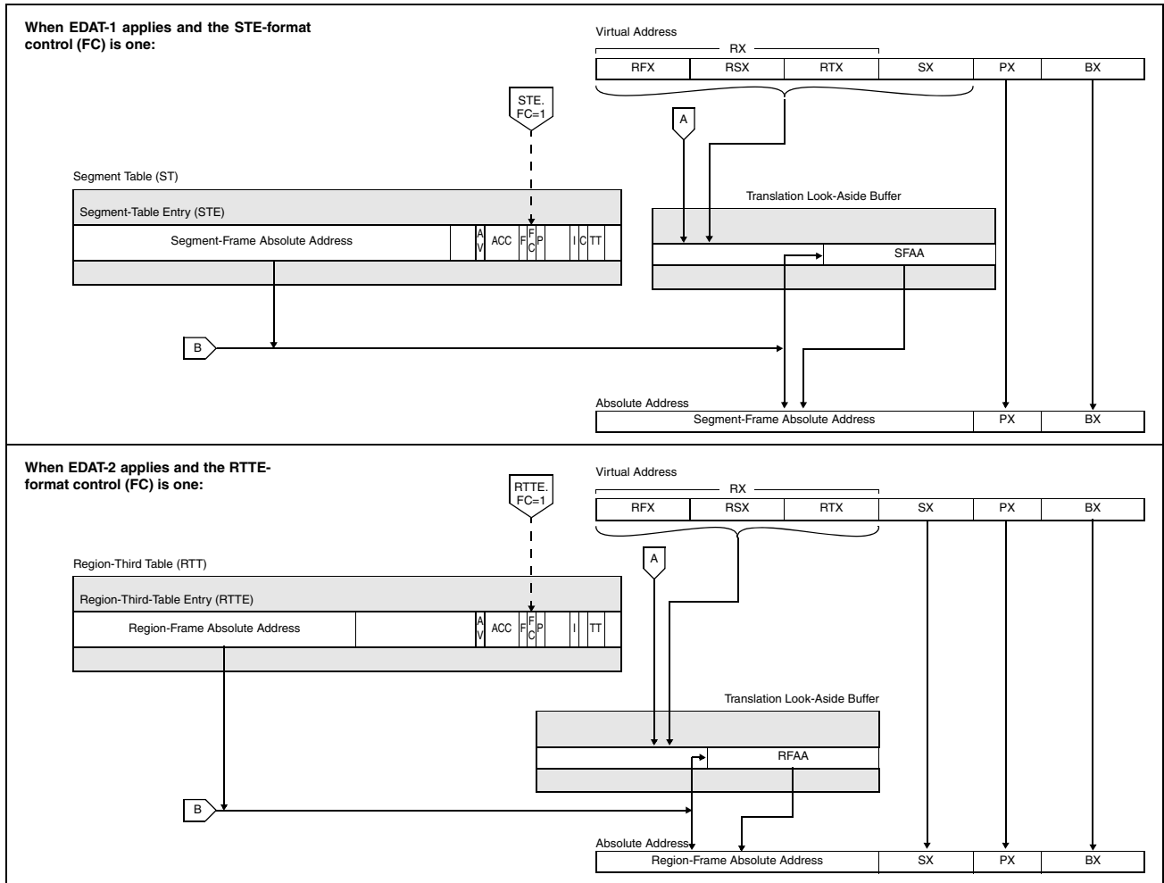
Figure 3-12. Translation Process (Part 3 of 3)
