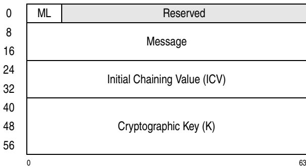
Figure 7-278. Parameter Block for PCC-Compute-Last-Block-CMAC-Using-AES-192
