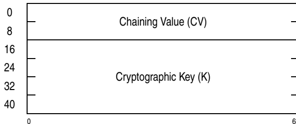
Figure 7-169. Parameter Block for KMO-AES-256
