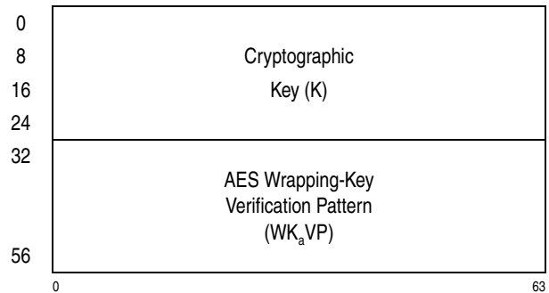
Figure 10-46. Parameter Block for PCKMO-Encrypt-AES-256-Key
