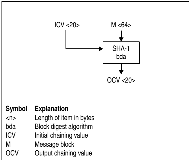
Figure 7-189. Symbol for SHA-1 Block Digest Algorithm
