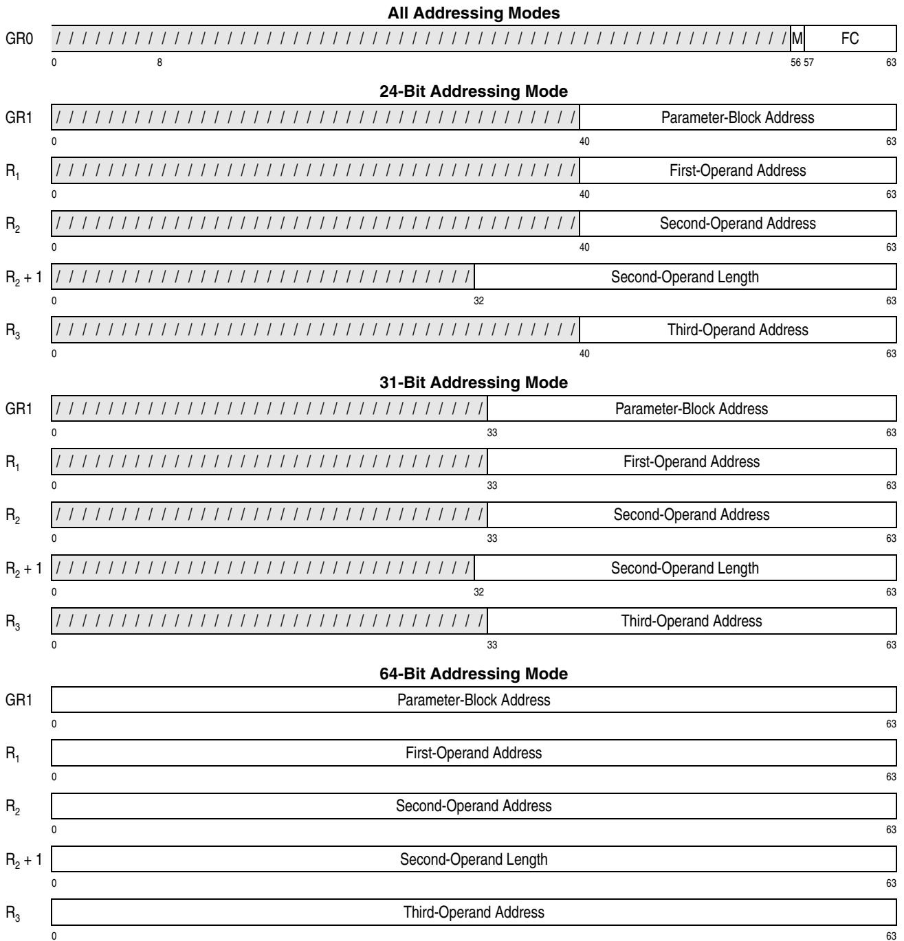
Figure 7-109. General Register Assignment for KMCTR
