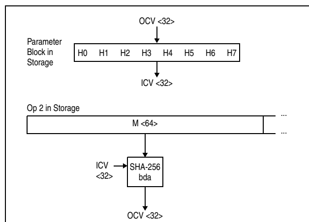
Figure 7-209. KLMD-SHA-256 Full Block ( L \geq 64 )
