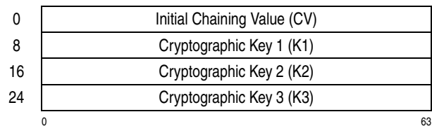
Figure 7-233. Parameter Block for KMAC-TDEA-192
