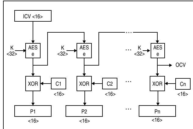
Figure 7-172. KMO-AES-256 Decipher Operation
