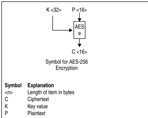
Figure 7-81. Symbols for AES-256 Encryption
