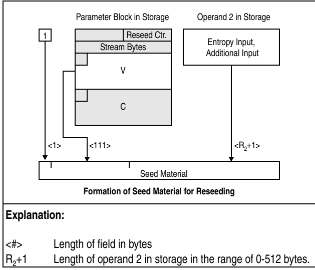
Figure 7-300. PPNO-SHA-512-DRNG Seed Operation's Generation of Seed Material (Part 2 of 2)
