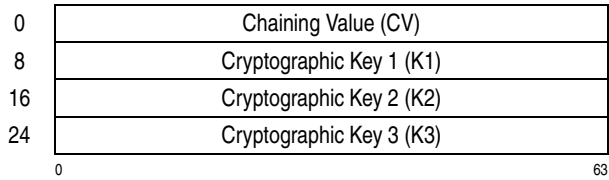
Figure 7-91. Parameter Block for KMF-TDEA-192
