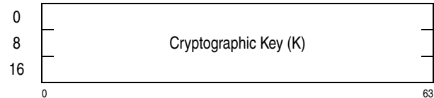
Figure 7-132. Parameter Block for KMCTR-AES-192
