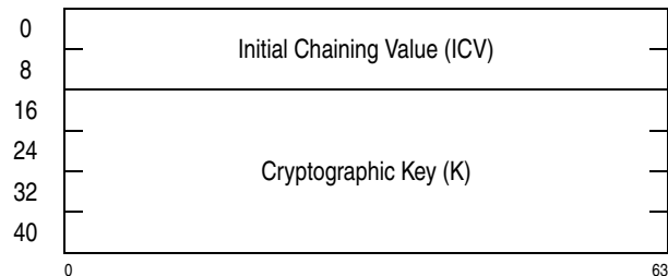
Figure 7-242. Parameter Block for KMAC-AES-256
