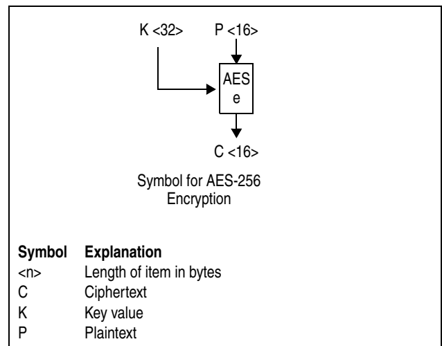
Figure 7-147. Symbols for AES-256 Encryption
