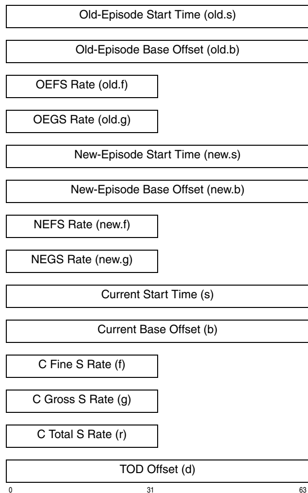
Figure 4-12. TOD-Clock-Steering Registers
