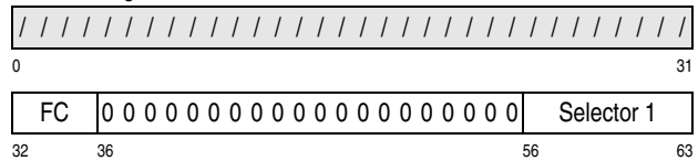
General Register 1
