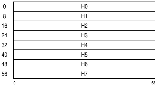
Figure 7-198. Parameter Block for KIMD-SHA-512
