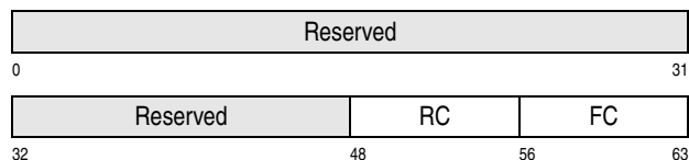
Figure 10-61. General-Register R_1 Format
