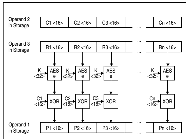
Figure 7-139. KMCTR AES Decipher Operation Using 256-Bit Key
