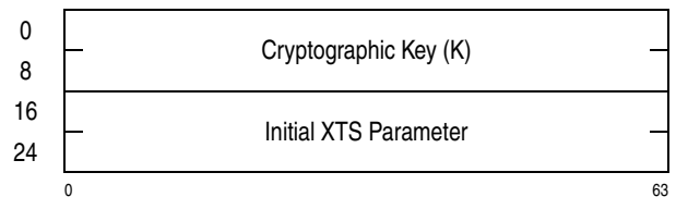
Figure 7-39. Parameter Block for KM-XTS-AES-128
