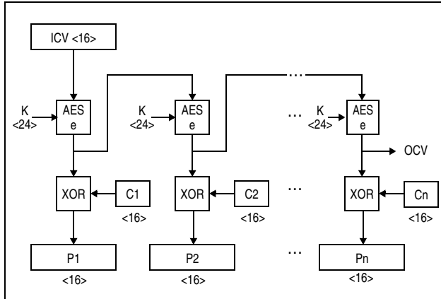
Figure 7-168. KMO-AES-192 Decipher Operation
