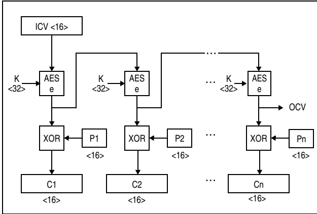
Figure 7-171. KMO-AES-256 Encipher Operation
