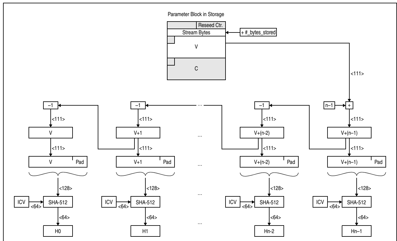
Figure 7-303. PPNO-SHA-512-DRNG Generate Operation's Generation of Deterministic Pseudorandom Numbers (Part 1 of 2)
