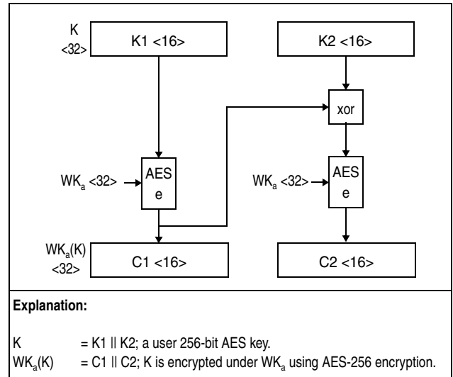
Figure 7-326. Encryption of 256-Bit AES Key Using WK_a
