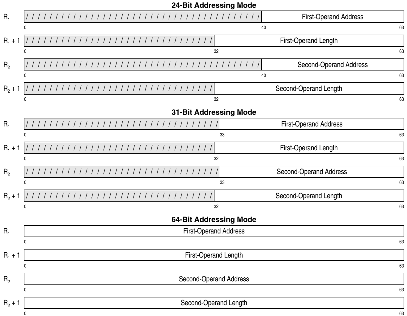
Figure 7-246. Register Contents for CONVERT UTF-16 TO UTF-32
