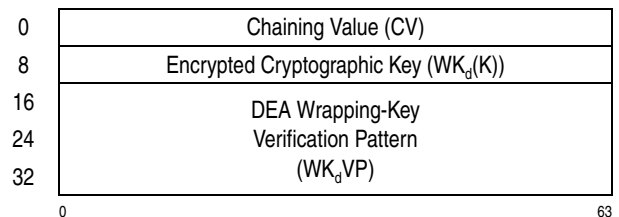
Figure 7-84. Parameter Block for KMF-Encrypted-DEA
