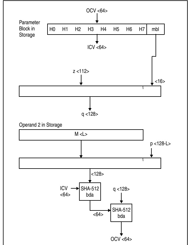
Figure 7-217. KLMD-SHA-512 Partial-Block Case 2 ( 112 \leq L \leq 127 )
