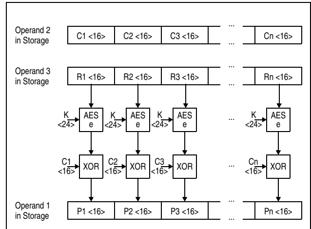
Figure 7-135. KMCTR AES Decipher Operation Using 192-Bit Key
