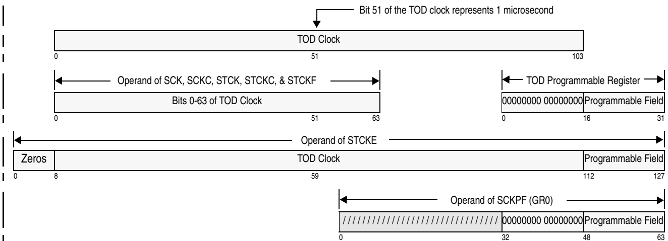
Figure 4-10. Format of the TOD Clock and TOD-Programmable Field as Set and Inspected by Various Instructions
