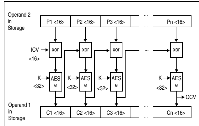
Figure 7-70. KMC AES Encipher Operation Using 256-Bit Key
