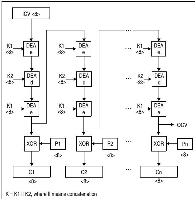
Figure 7-155. KMO-TDEA-128 Encipher Operation
