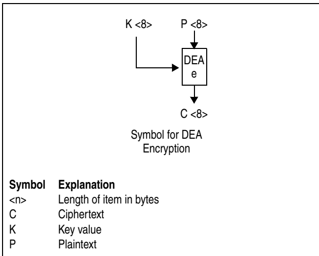
Figure 7-111. Symbols for DEA Encryption
