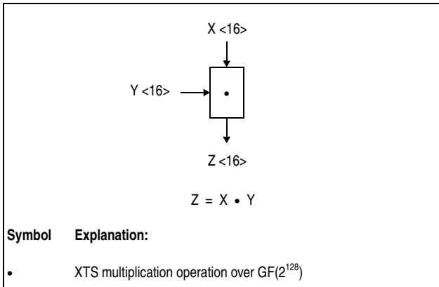
Figure 7-9. Symbol For XTS Multiplication Operation Over GF(2^{128})
