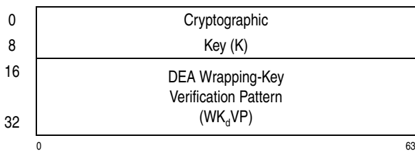
Figure 10-42. Parameter Block for PCKMO-Encrypt-TDEA-128-Key
