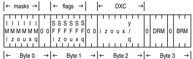
Figure 9-5. FPC Register Overview
