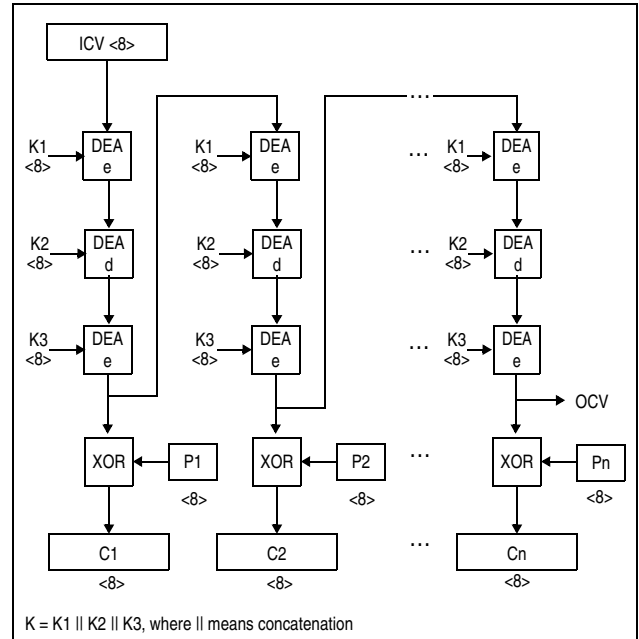
Figure 7-159. KMO-TDEA-192 Encipher Operation
