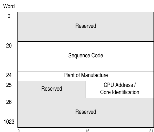
Figure 10-76. Format of the SYSIB 1.2.1
