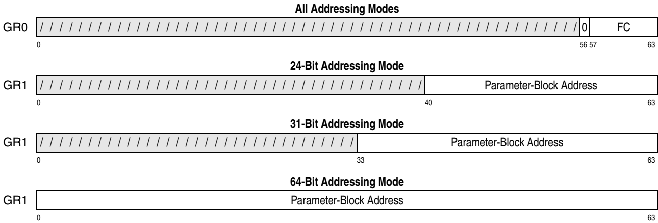
Figure 10-48. General Register Assignment for PERFORM TIMING FACILITY FUNCTION
