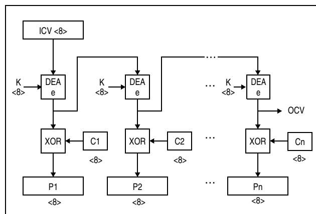
Figure 7-152. KMO-DEA Decipher Operation
