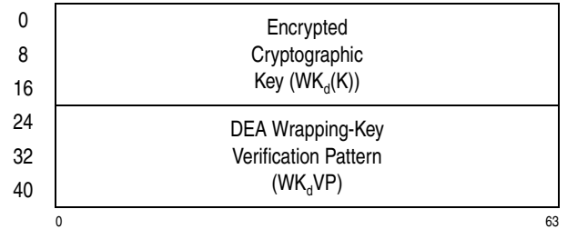
Figure 7-24. Parameter Block for KM-Encrypted-TDEA-192
