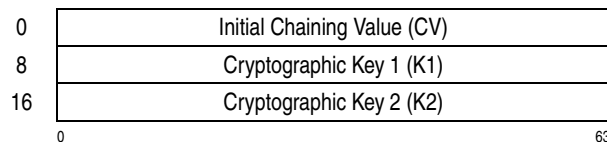
Figure 7-230. Parameter Block for KMAC-TDEA-128
