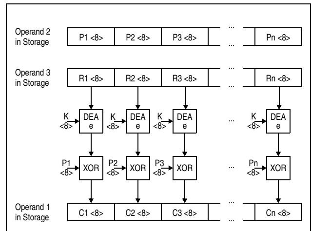
Figure 7-118. KMCTR DEA Encipher Operation Using 64-Bit Key
