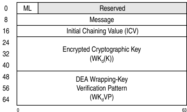
Figure 7-273. Parameter Block for PCC-Compute-Last-Block-CMAC-Using-Encrypted-TDEA-192
