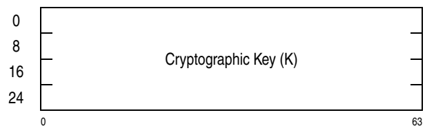
Figure 7-136. Parameter Block for KMCTR-AES-256
