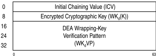
Figure 7-228. Parameter Block for KMAC-Encrypted-DEA
