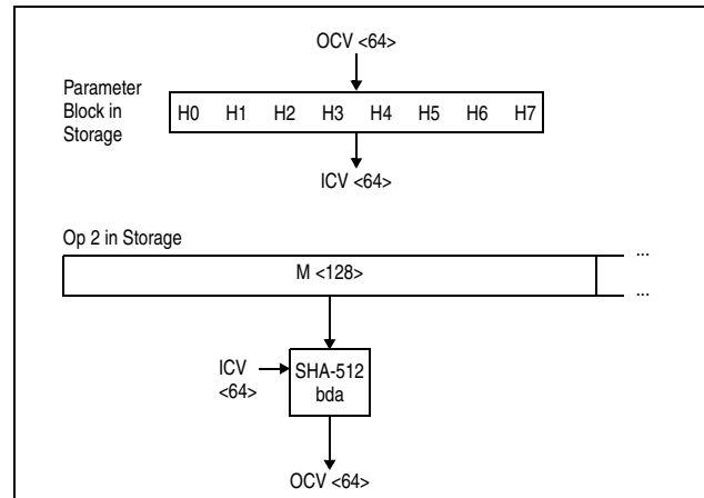
Figure 7-214. KLMD-SHA-512 Full Block ( L \geq 128 )
