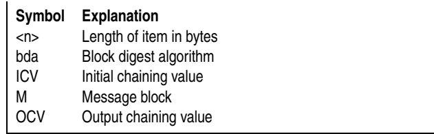
Figure 7-191. Symbol for SHA-512 Block Digest Algorithm
