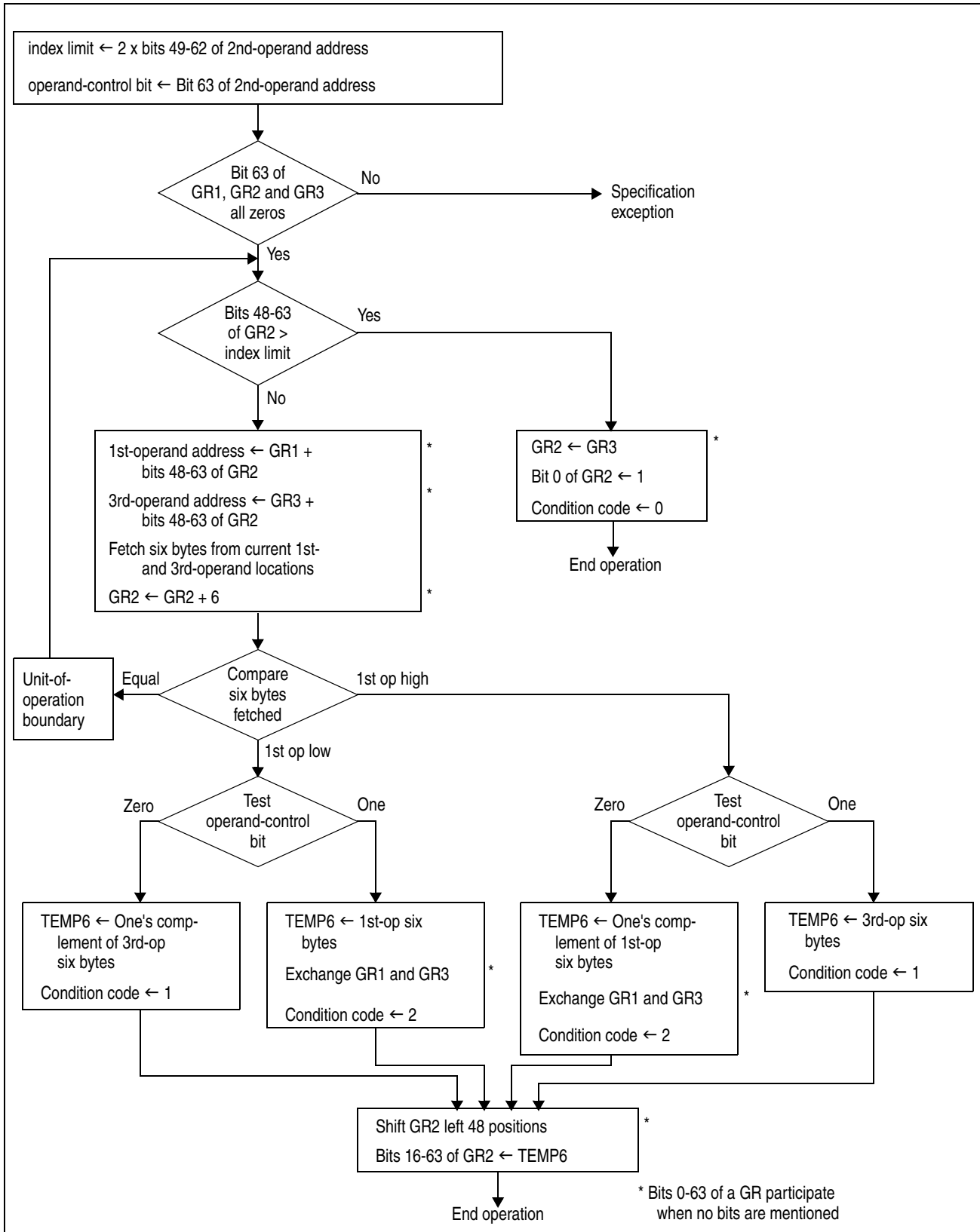
Figure 7-177. Execution of COMPARE AND FORM CODEWORD in the 64-bit Addressing Mode
