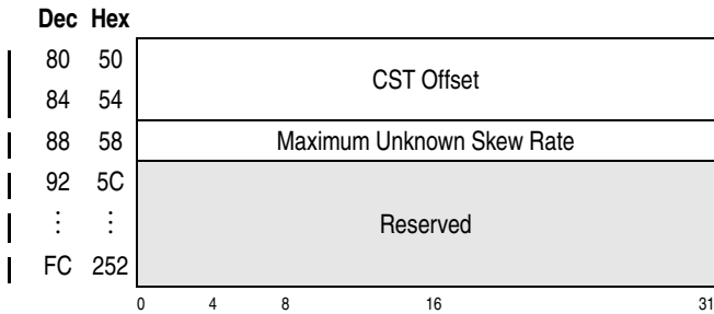
Figure 4-13. UTC Information Block
