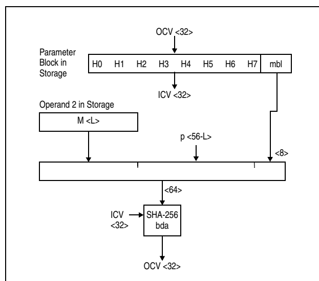
Figure 7-211. KLMD-SHA-256 Partial-Block Case 1 ( 1 \leq L \leq 55 )
