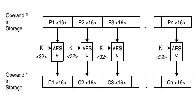
Figure 7-37. KM AES Encipher Operation Using 256-Bit Key
