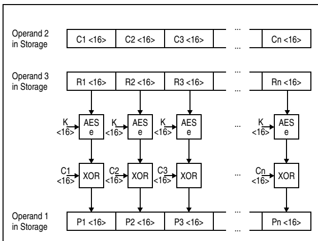
Figure 7-131. KMCTR AES Decipher Operation Using 128-Bit Key
