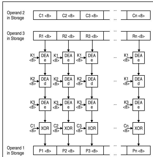
Figure 7-127. KMCTR TDEA Decipher Operation Using 192-Bit Key
