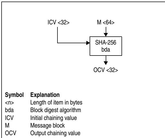
Figure 7-190. Symbol for SHA-256 Block Digest Algorithm
