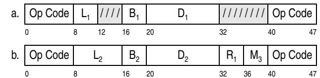
Figure 5-1. Basic Instruction Formats (Part 2 of 5)
