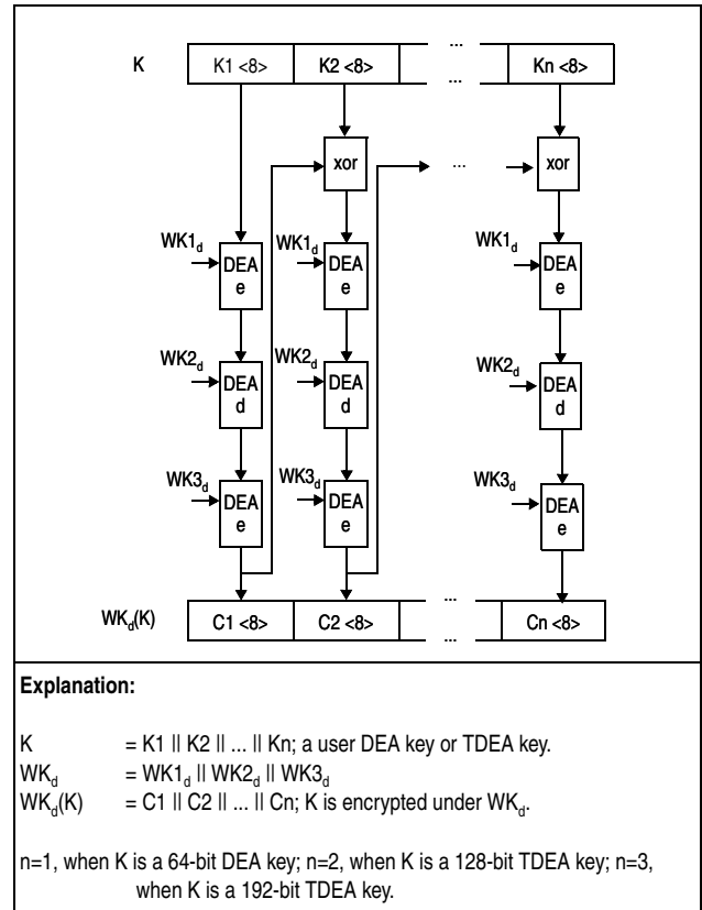
Figure 7-320. Encryption of DEA or TDEA Key Using WK_d
