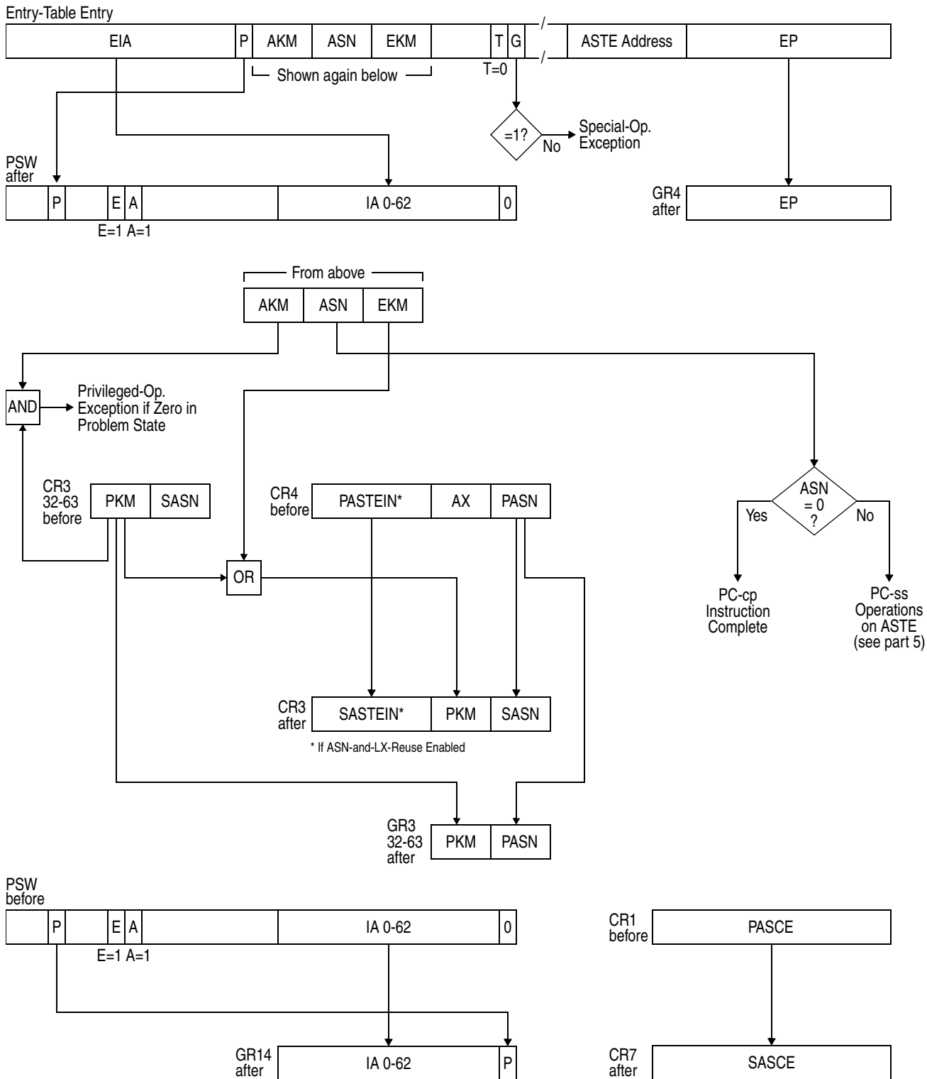
Figure 10-63. Execution of PROGRAM CALL (Part 2 of 5).
