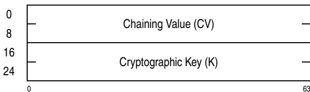
Figure 7-161. Parameter Block for KMO-AES-128
