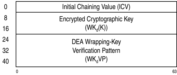
Figure 7-231. Parameter Block for KMAC-Encrypted-TDEA-128
