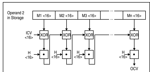
Figure 7-201. KIMD-GHASH
