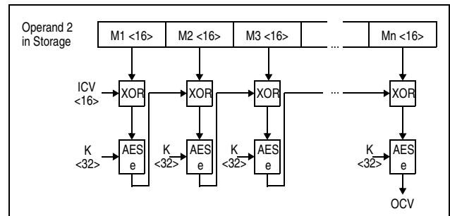
Figure 7-244. KMAC-AES-256
