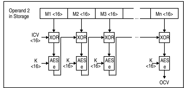
Figure 7-238. KMAC-AES-128
