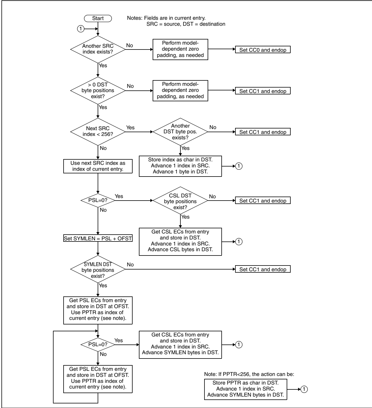
Figure 7-185. Expansion Process
