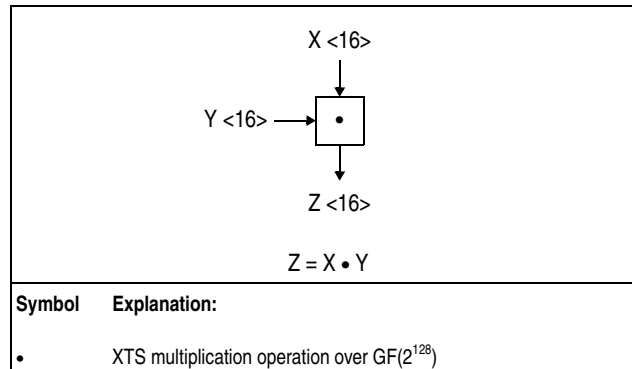
Figure 7-259. Symbol For XTS Multiplication Operation Over GF(2^{128})
