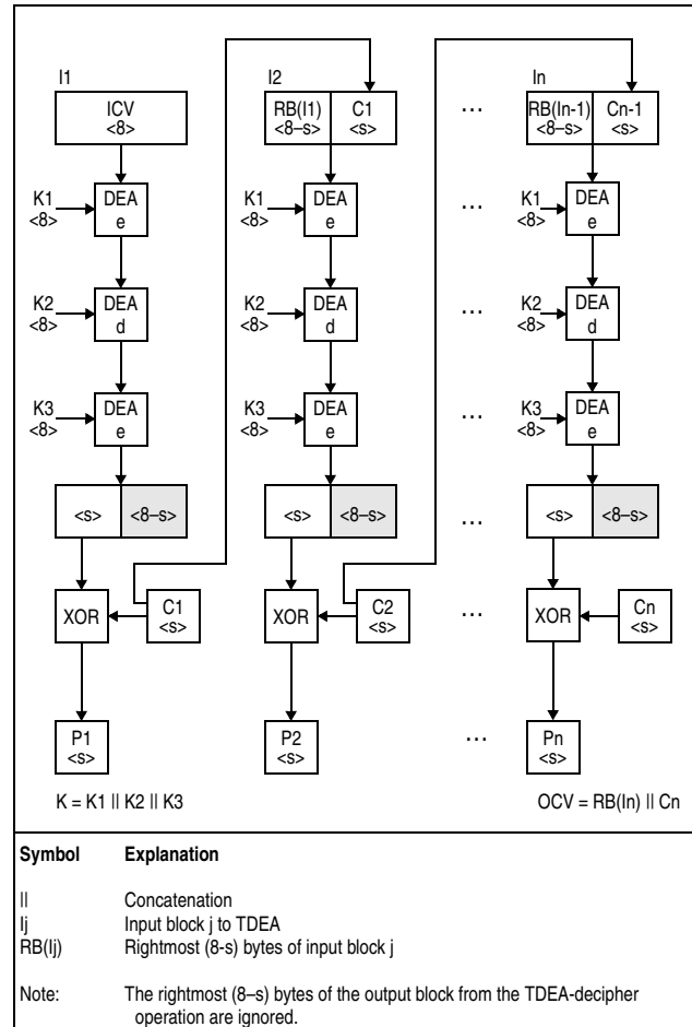
Figure 7-94. KMF-TDEA-192 Decipher Operation
