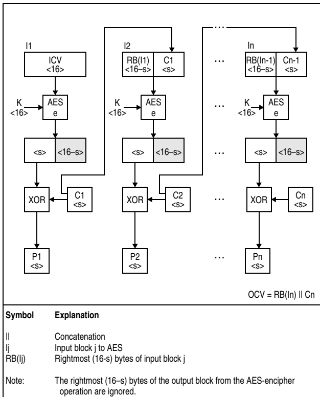
Figure 7-98. KMF-AES-128 Decipher Operation
