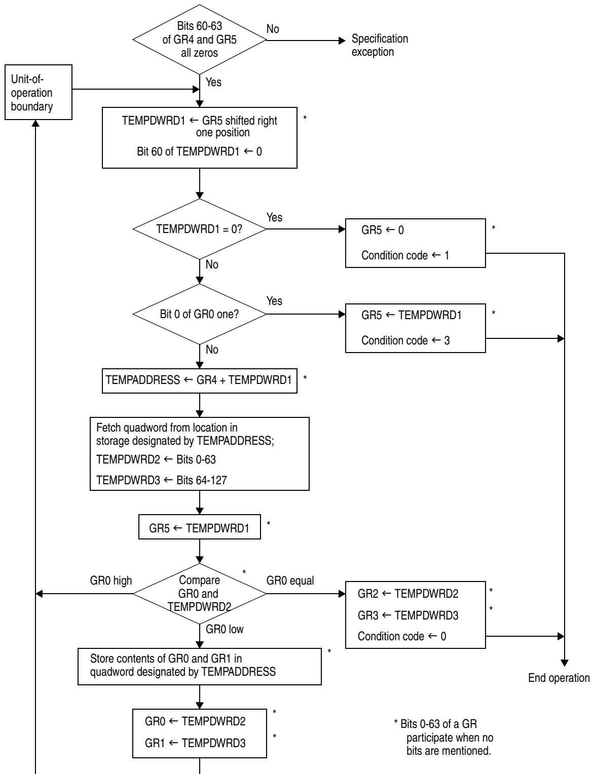
Figure 7-315. Execution of UPDATE TREE in the 64-Bit Addressing Mode
