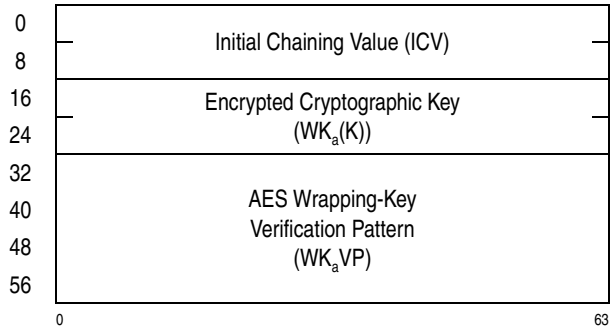
Figure 7-237. Parameter Block for KMAC-Encrypted-AES-128
