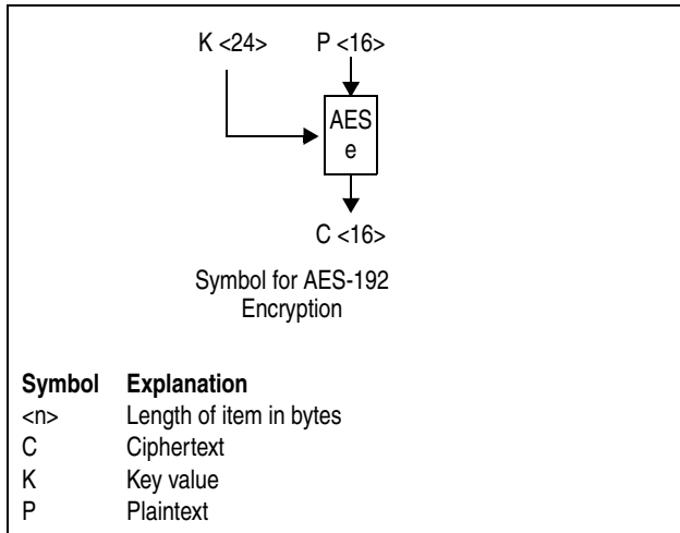
Figure 7-80. Symbols for AES-192 Encryption
