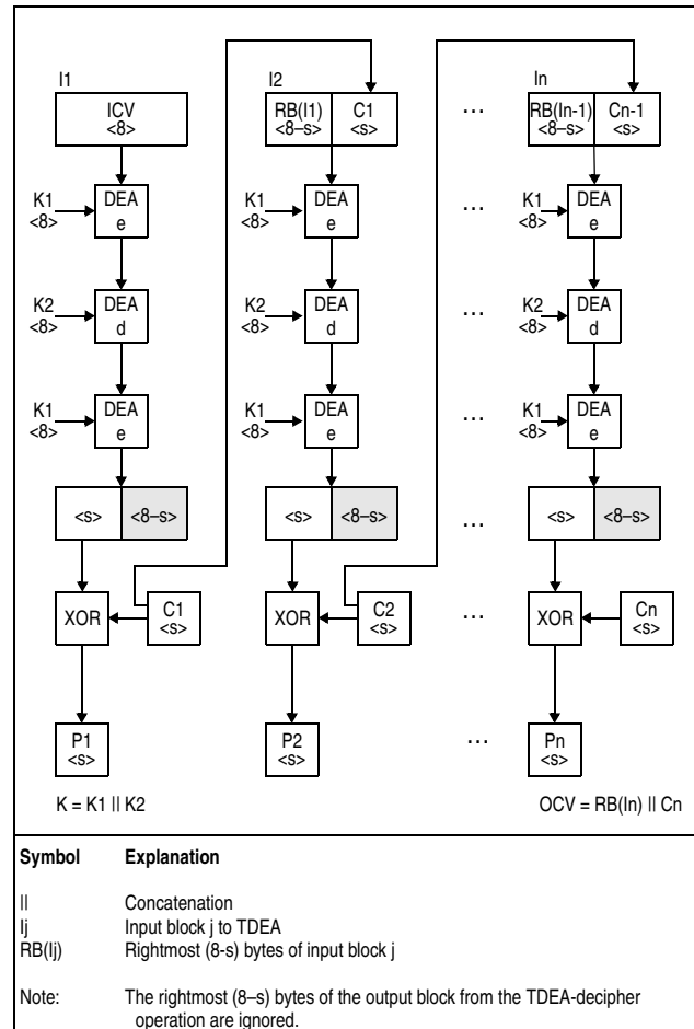
Figure 7-90. KMF-TDEA-128 Decipher Operation
