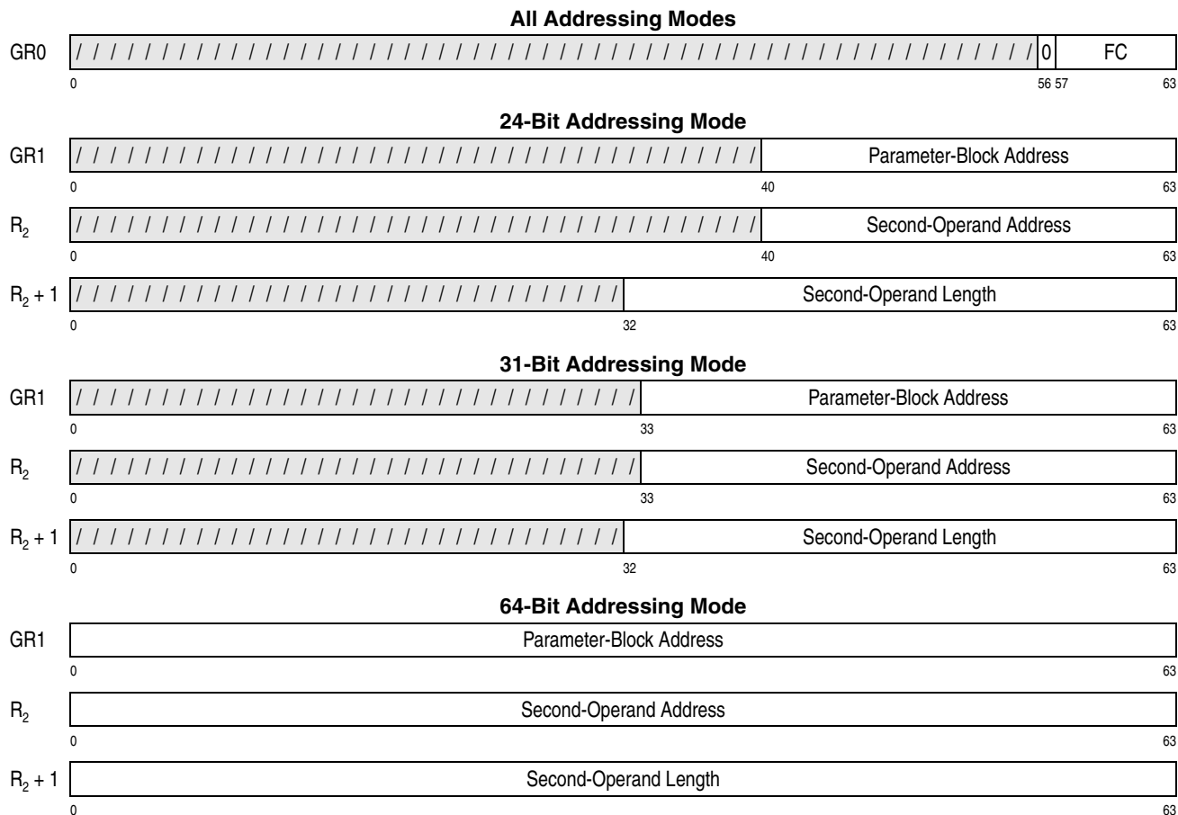
Figure 7-188. General Register Assignment for KIMD and KLMD
