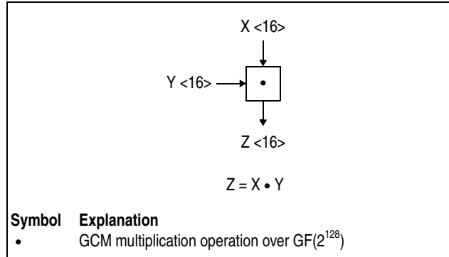
Figure 7-192. Symbol For GCM Multiplication Operation Over GF(2^{128})
