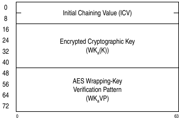
Figure 7-243. Parameter Block for KMAC-Encrypted-AES-256
