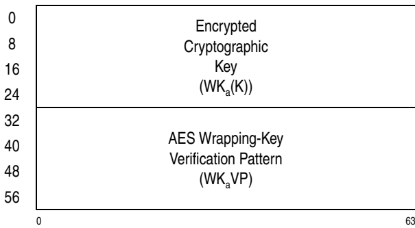
Figure 7-137. Parameter Block for KMCTR-Encrypted-AES-256
