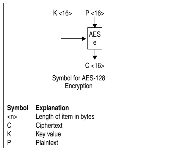
Figure 7-79. Symbols for AES-128 Encryption
