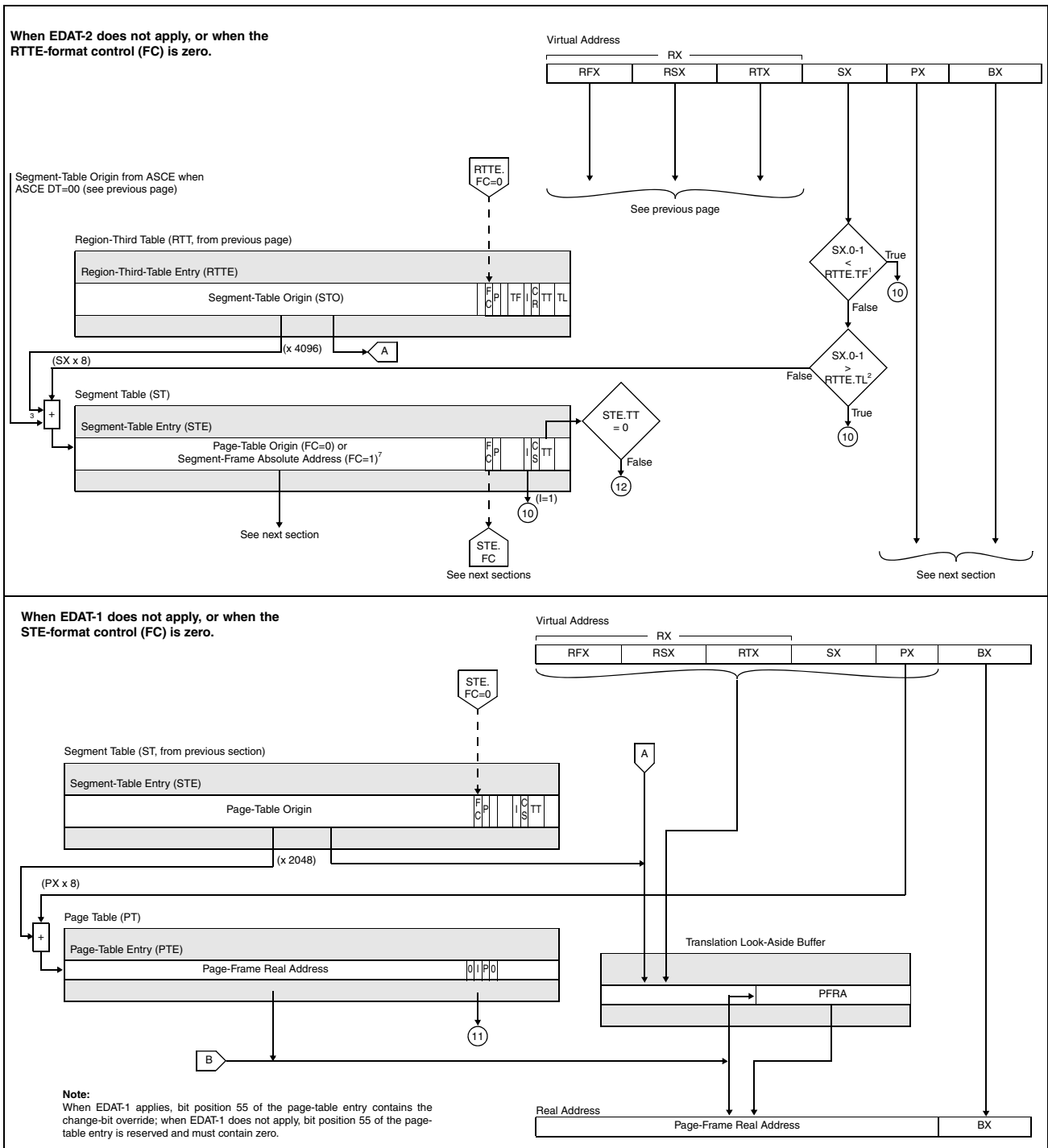
Figure 3-12. Translation Process (Part 2 of 3)
