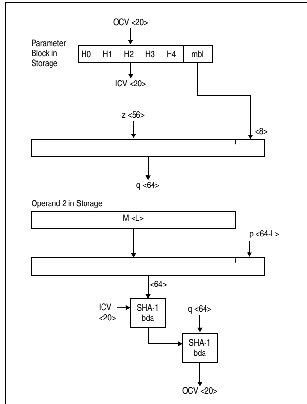
Figure 7-207. KLMD-SHA-1 Partial-Block Case 2 ( 56 \leq L \leq 63 )
