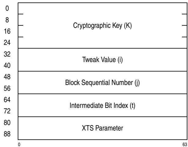
Figure 7-287. Parameter Block for PCC-Compute-XTS-Parameter-Using-AES-256
