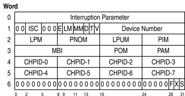
Figure 15-1. PMCW Format
