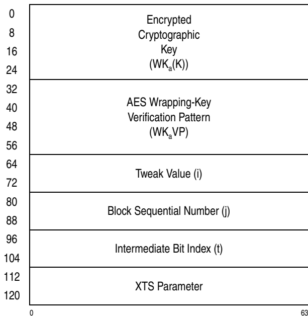
Figure 7-288. Parameter Block for PCC-Compute-XTS-Parameter-Using-Encrypted-AES-256
