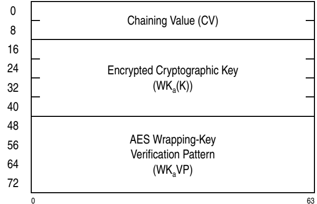
Figure 7-170. Parameter Block for KMO-AES-256
