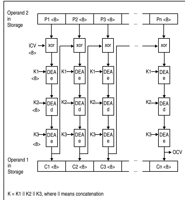
Figure 7-58. KMC TDEA Encipher Operation Using 192-Bit Key
