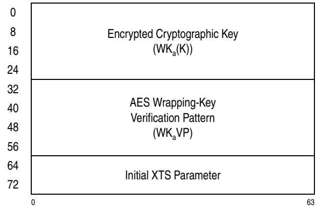
Figure 7-44. Parameter Block for KM-XTS-Encrypted-AES-256
