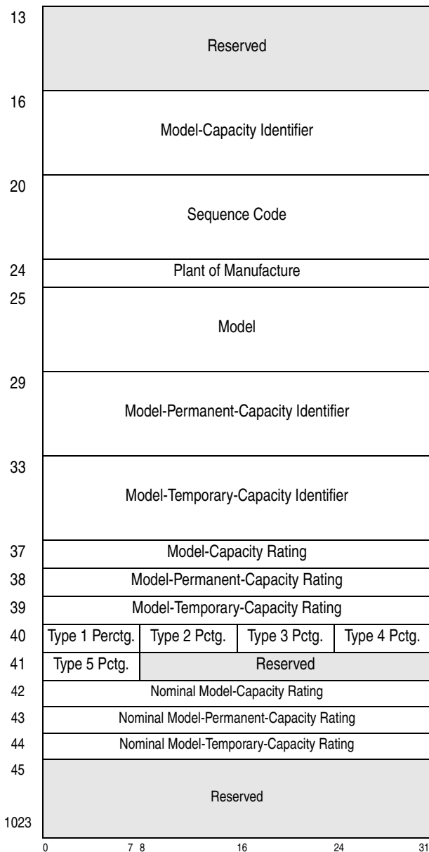
Figure 10-75. Format of the SYSIB 1.1.1 (Part 2 of 2)
