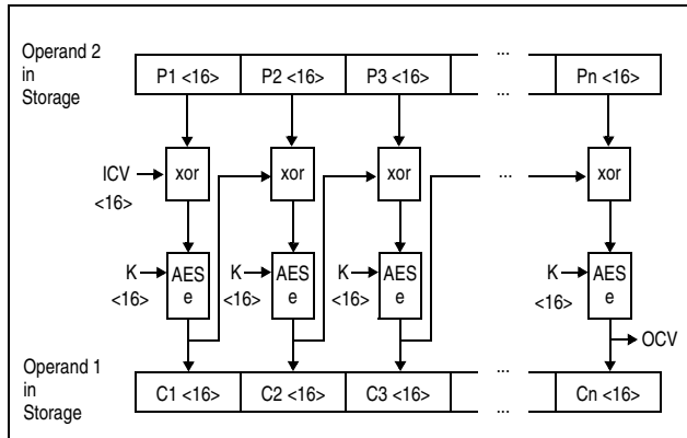
Figure 7-62. KMC AES Encipher Operation Using 128-Bit Key
