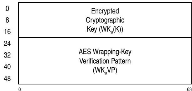
Figure 7-133. Parameter Block for KMCTR-Encrypted-AES-192
