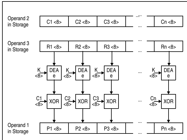
Figure 7-119. KMCTR DEA Decipher Operation Using 64-Bit Key
