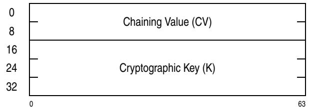
Figure 7-165. Parameter Block for KMO-AES-192
