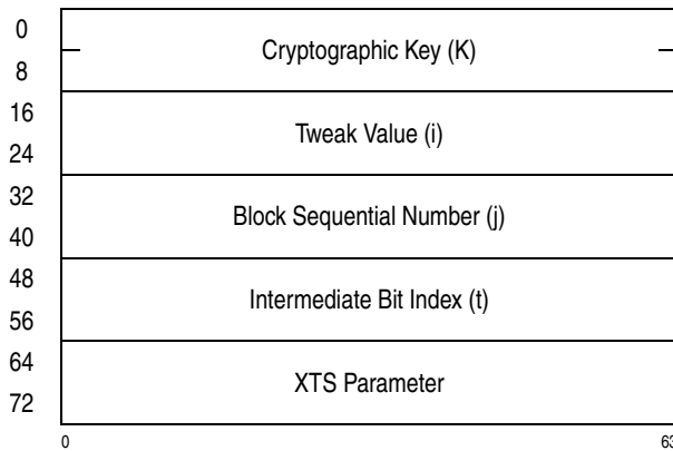
Figure 7-284. Parameter Block for PCC-Compute-XTS-Parameter-Using-AES-128
