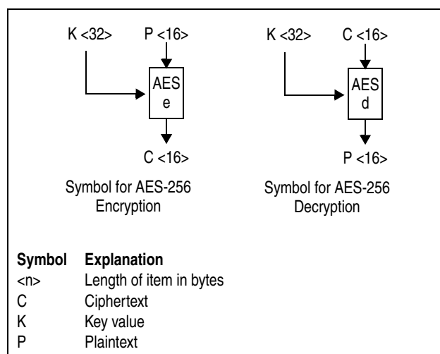
Figure 7-264. Symbols for AES-256 Encryption and Decryption
