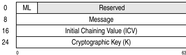
Figure 7-266. Parameter Block for PCC-Compute-Last-Block-CMAC-Using-DEA
