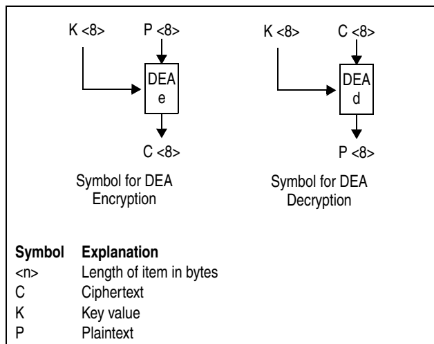
Figure 7-222. Symbols for DEA Encryption and Decryption
