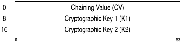
Figure 7-52. Parameter Block for KMC-TDEA-128
