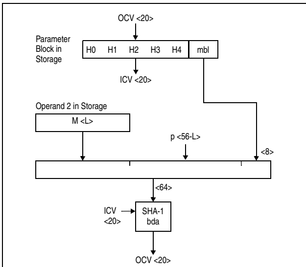
Figure 7-206. KLMD-SHA-1 Partial-Block Case 1 ( 1 \leq L \leq 55 )
