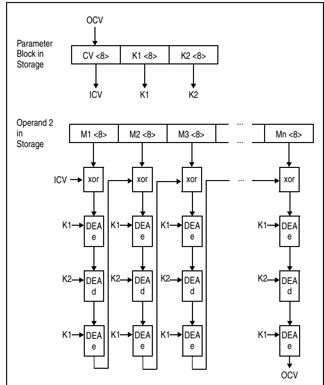
Figure 7-232. MAC Computation Using 128-bit TDEA Key
