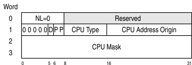
Figure 10-84. CPU-Type Topology-List Entry
