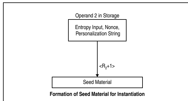
Figure 7-300. PPNO-SHA-512-DRNG Seed Operation's Generation of Seed Material (Part 1 of 2)
