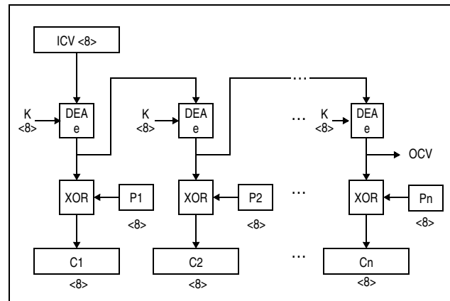
Figure 7-151. KMO-DEA Encipher Operation
