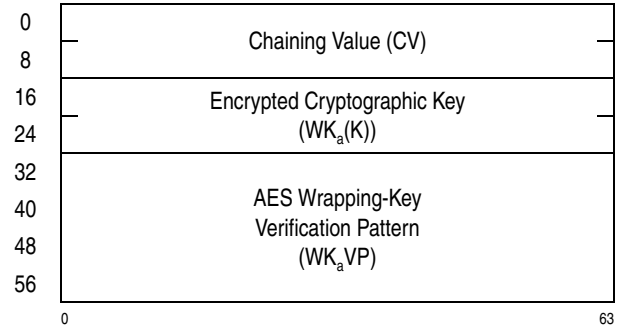
Figure 7-61. Parameter Block for KMC-Encrypted-AES-128
