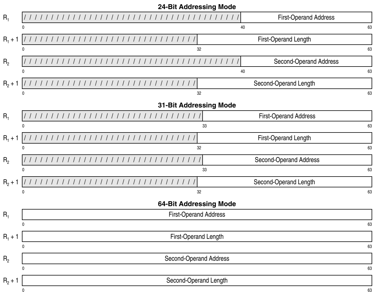
Figure 7-250. Register Contents for CONVERT UTF-8 TO UTF-16
