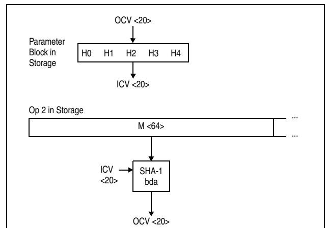
Figure 7-204. KLMD-SHA-1 Full Block ( L \geq 64 )
