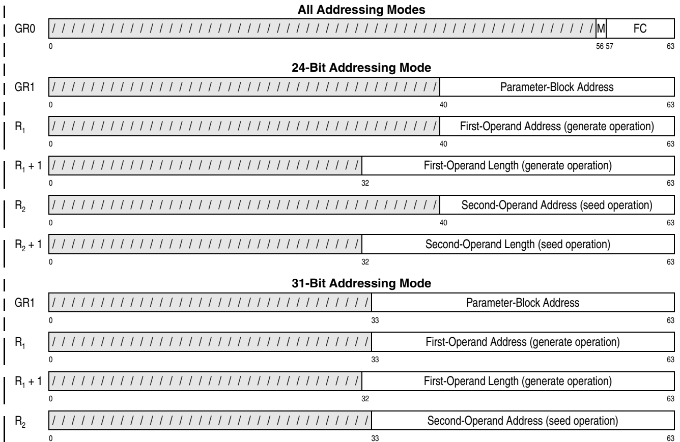
Figure 7-297. General Register Assignment for PPNO (Part 1 of 2)
