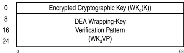
Figure 7-117. Parameter Block for KMCTR-Encrypted-DEA
