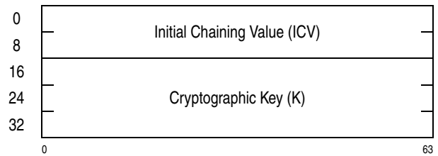
Figure 7-239. Parameter Block for KMAC-AES-192
