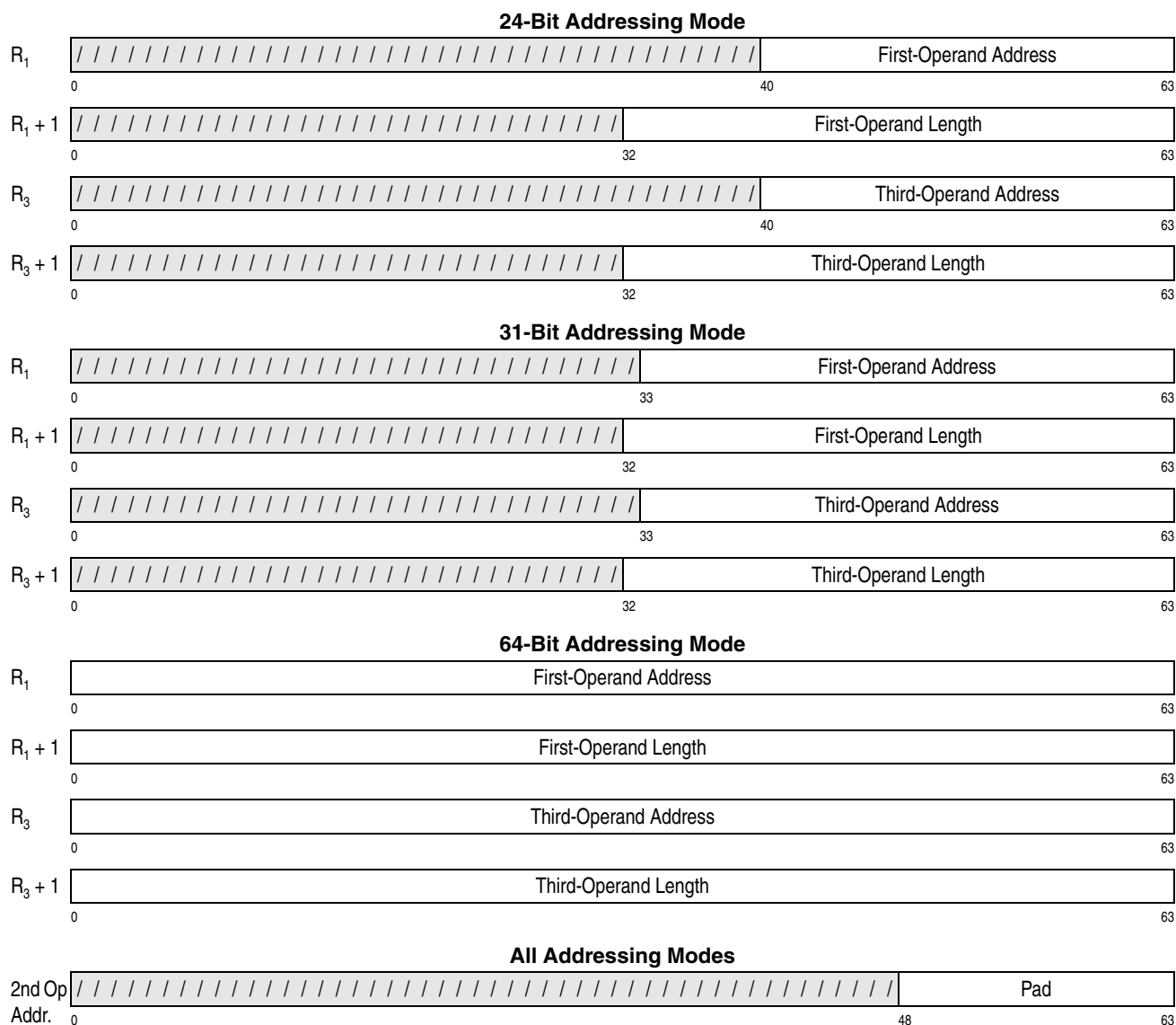
Figure 7-181. Register Contents and Second-Operand Address for COMPARE LOGICAL LONG UNICODE
