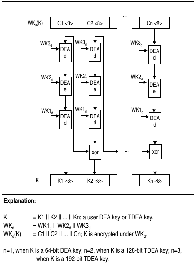
Figure 7-321. Decryption of DES or TDES Key Using WK_d
