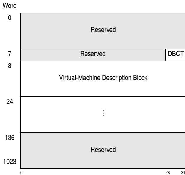
Figure 10-80. Format of the SYSIB 3.2.2
