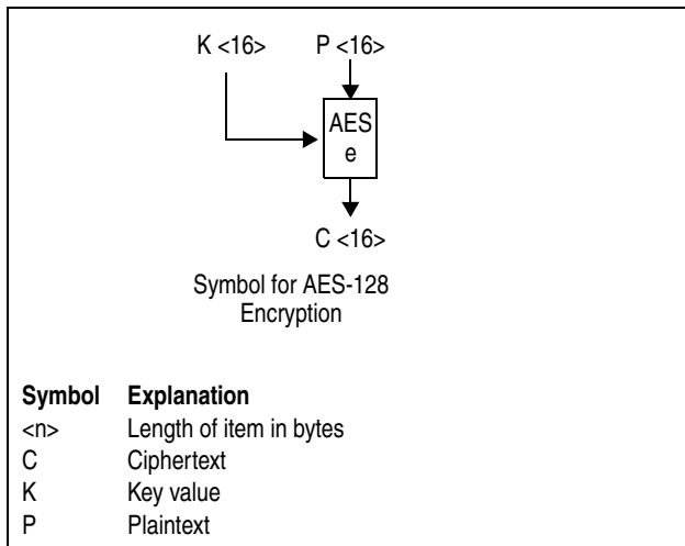
Figure 7-145. Symbols for AES-128 Encryption
