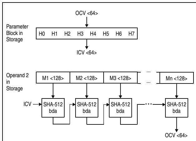
Figure 7-199. KIMD-SHA-512
