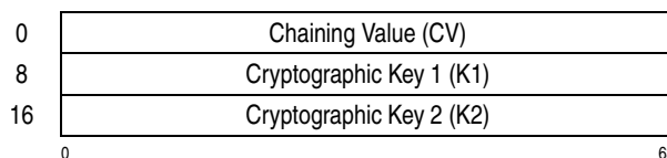
Figure 7-87. Parameter Block for KMF-TDEA-128
