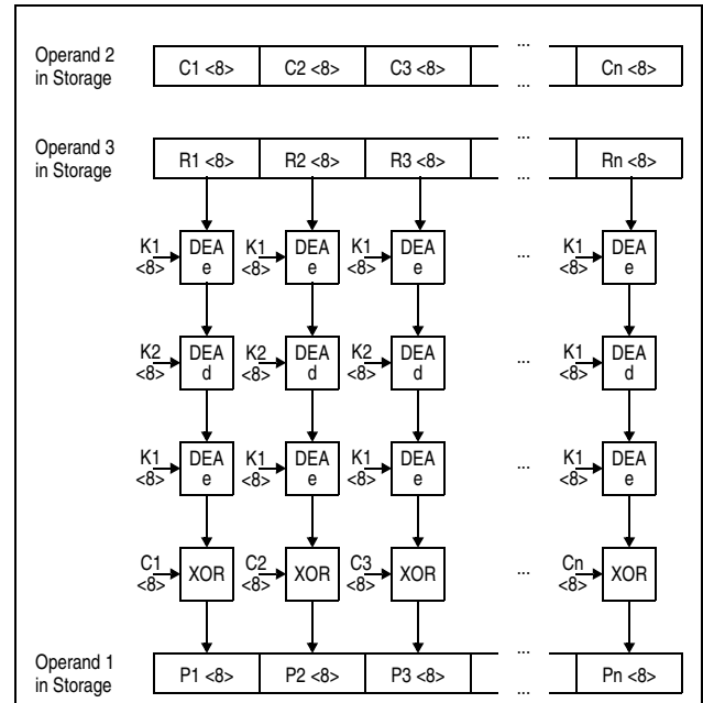
Figure 7-123. KMCTR TDEA Decipher Operation Using 128-Bit Key
