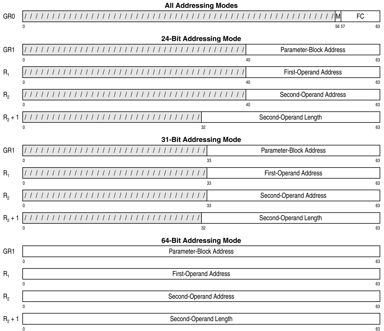
Figure 7-142. General Register Assignment for KMO
