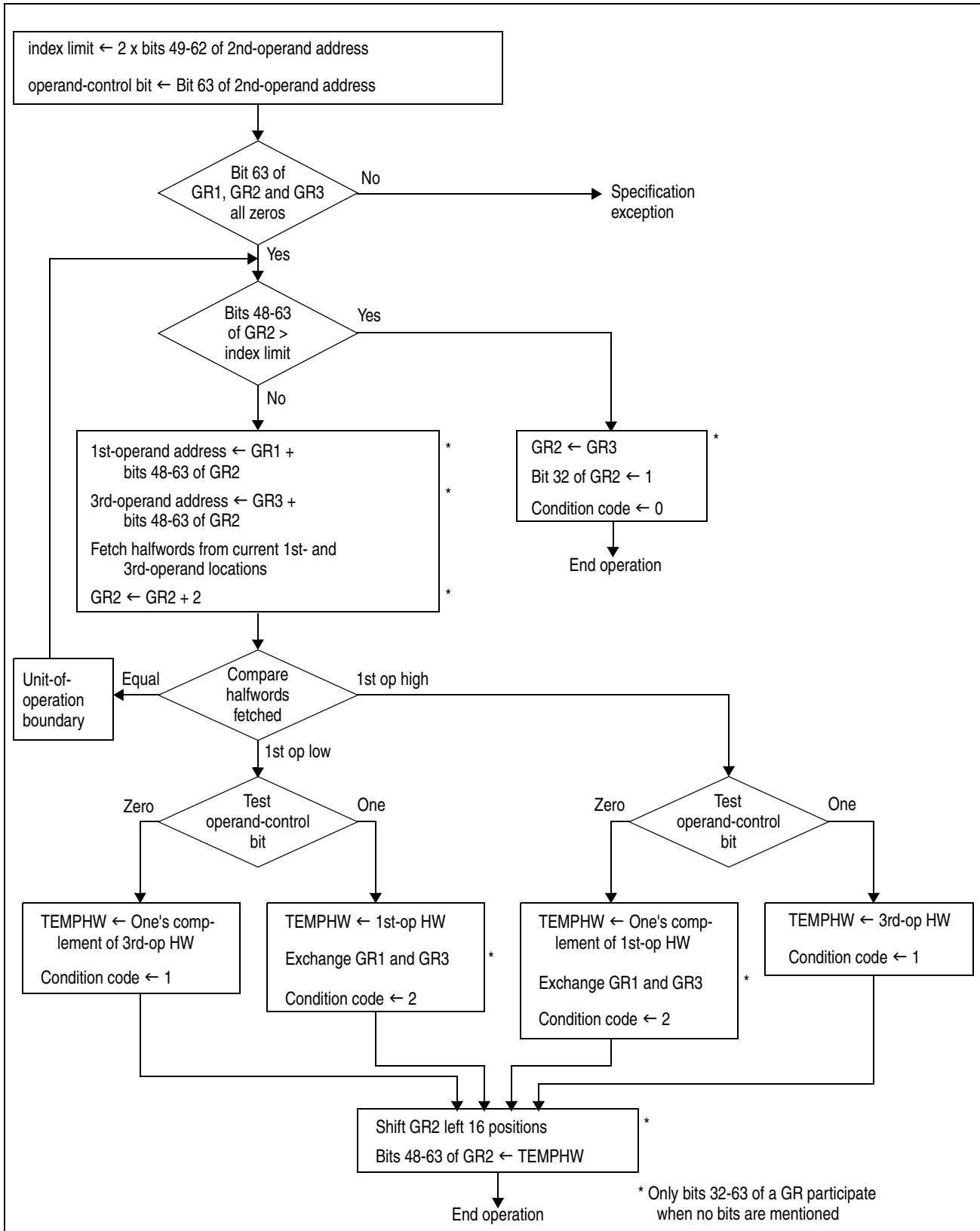
Figure 7-175. Execution of COMPARE AND FORM CODEWORD in the 24-bit or 31-bit Addressing Mode
