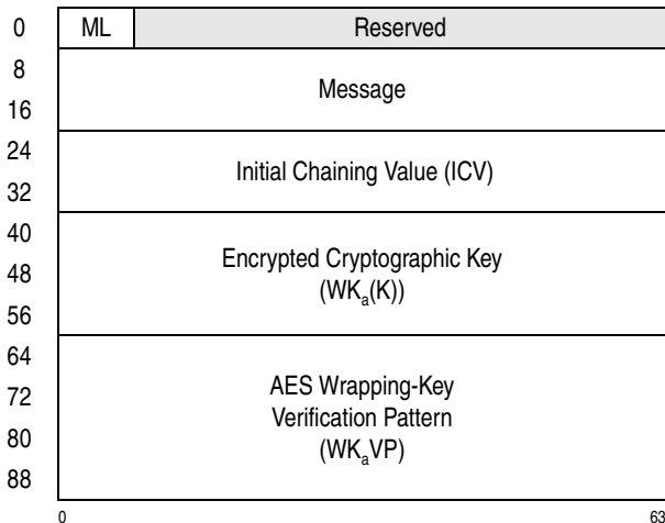
Figure 7-279. Parameter Block for PCC-Compute-Last-Block-CMAC-Using-Encrypted-AES-192
