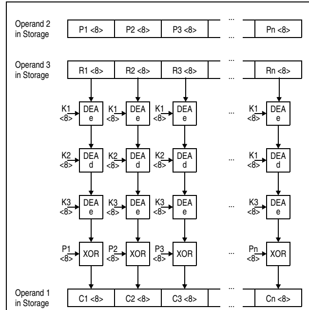
Figure 7-126. KMCTR TDEA Encipher Operation Using 192-Bit Key
