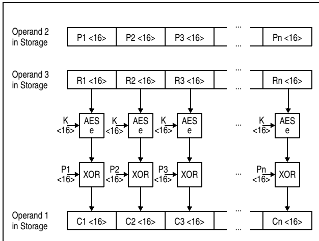
Figure 7-130. KMCTR AES Encipher Operation Using 128-Bit Key
