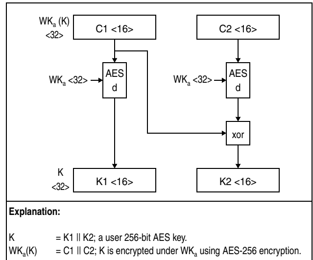
Figure 7-327. Decryption of 256-Bit AES Key Using WK_a
