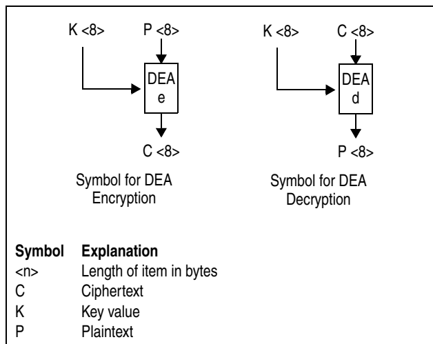
Figure 7-261. Symbols for DEA Encryption and Decryption
