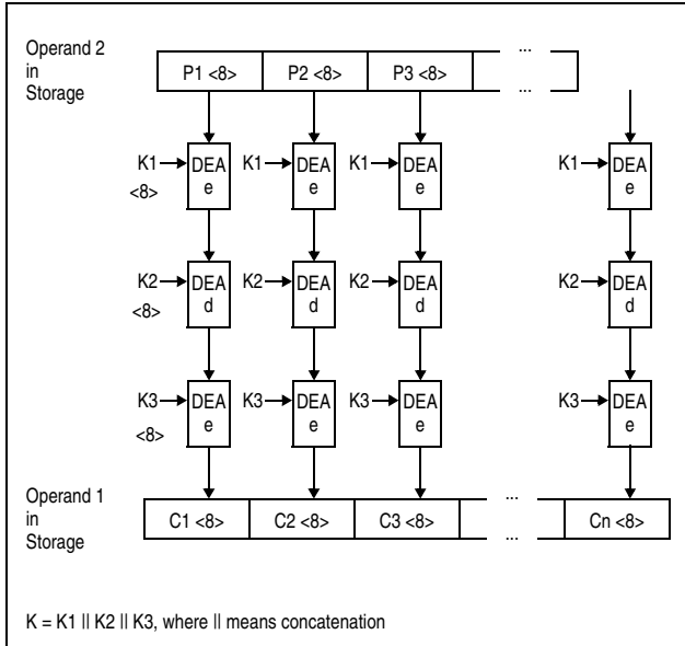
Figure 7-25. KM TDEA Encipher Operation Using 192-Bit Key
