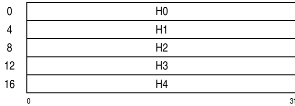
Figure 7-194. Parameter Block for KIMD-SHA-1
