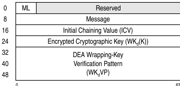
Figure 7-267. Parameter Block for PCC-Compute-Last-Block-CMAC-Using-Encrypted-DEA
