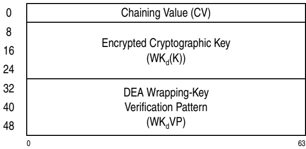
Figure 7-158. Parameter Block for KMO-Encrypted-TDEA-192
