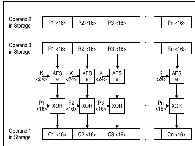
Figure 7-134. KMCTR AES Encipher Operation Using 192-Bit Key
