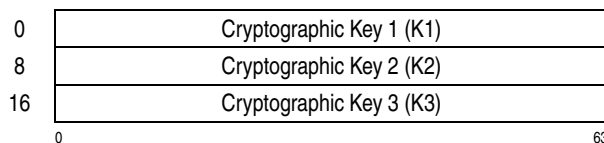
Figure 7-23. Parameter Block for KM-TDEA-192
