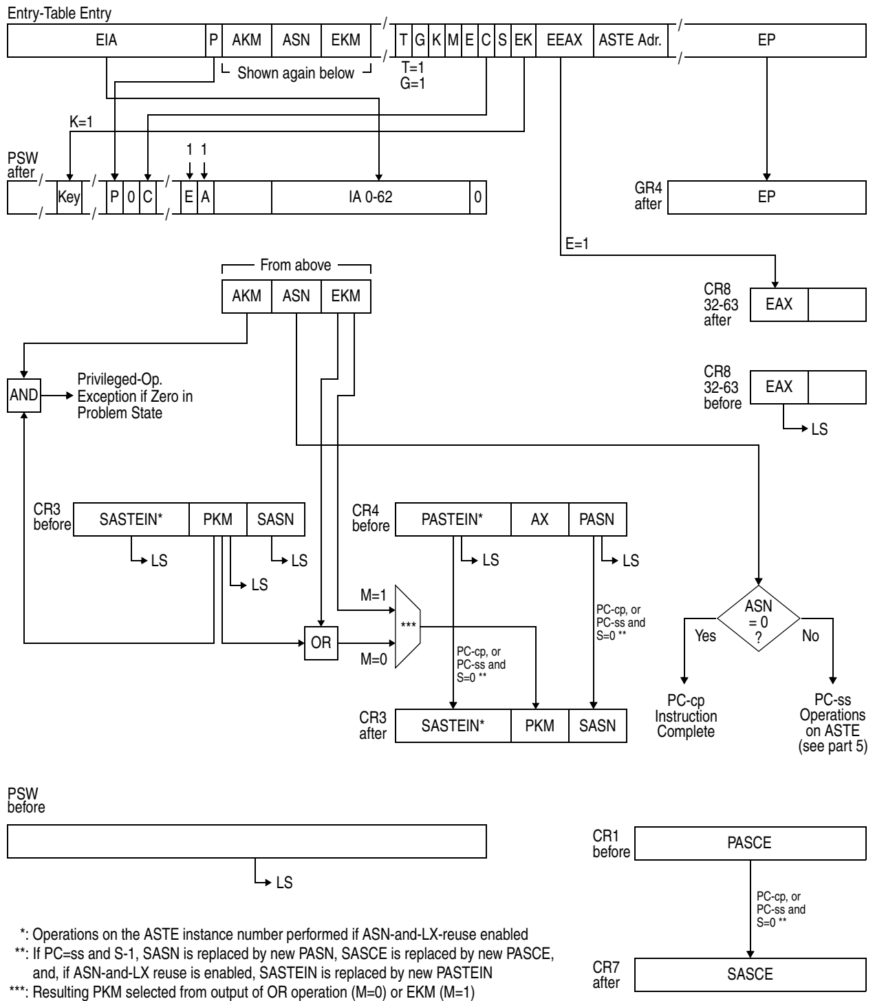
Figure 10-63. Execution of PROGRAM CALL (Part 3 of 5).
