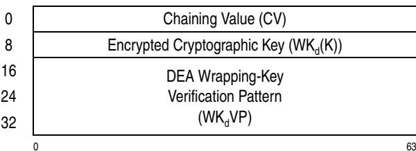
Figure 7-150. Parameter Block for KMO-Encrypted-DEA
