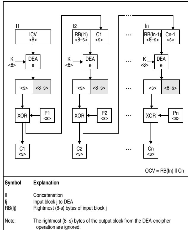
Figure 7-85. KMF-DEA Encipher Operation
