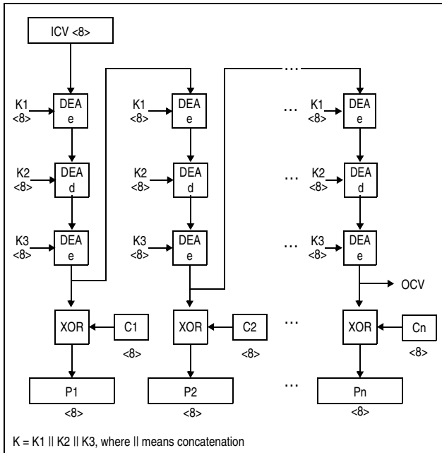
Figure 7-160. KMO-TDEA-192 Decipher Operation
