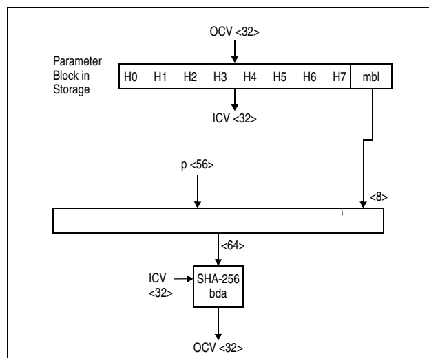
Figure 7-210. KLMD-SHA-256 Empty Block ( L = 0 )
