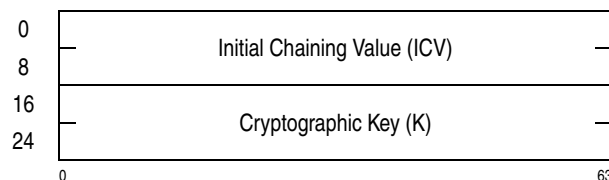
Figure 7-236. Parameter Block for KMAC-AES-128
