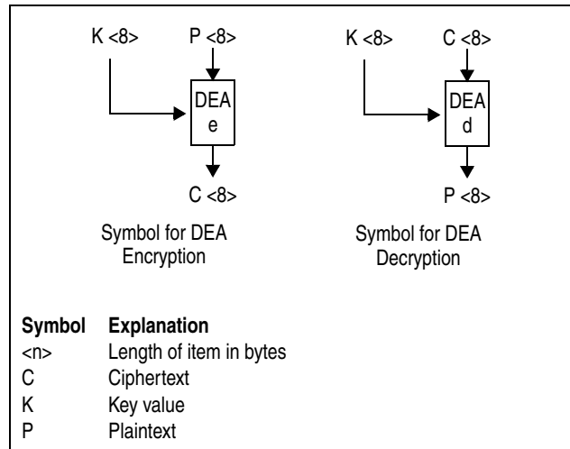
Figure 7-78. Symbols for DEA Encryption and Decryption
