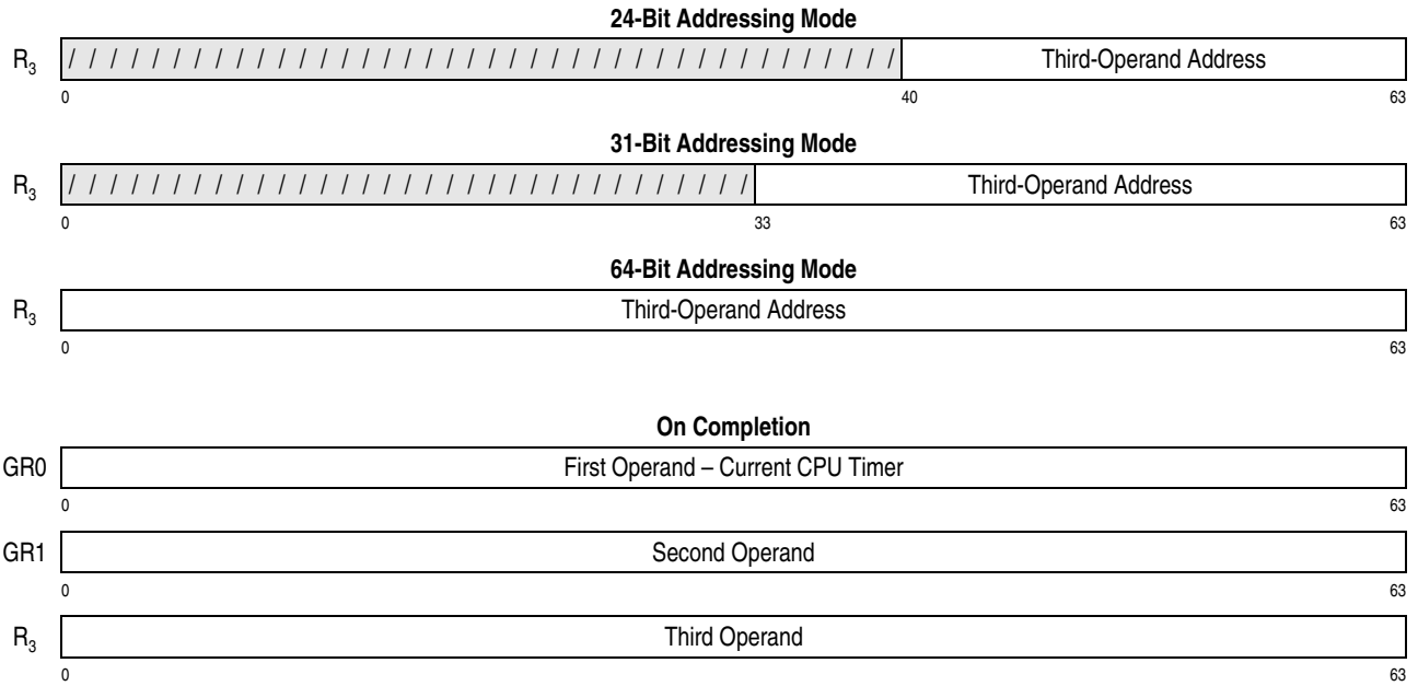
Figure 7-252. General Register Assignment for EXTRACT CPU TIME
