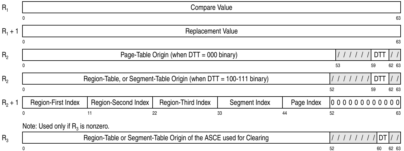
Figure 10-5. Register Contents for COMPARE AND REPLACE DAT TABLE ENTRY
