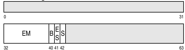
Control Register 10
