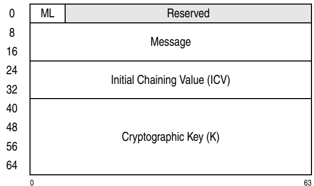
Figure 7-281. Parameter Block for PCC-Compute-Last-Block-CMAC-Using-AES-256
