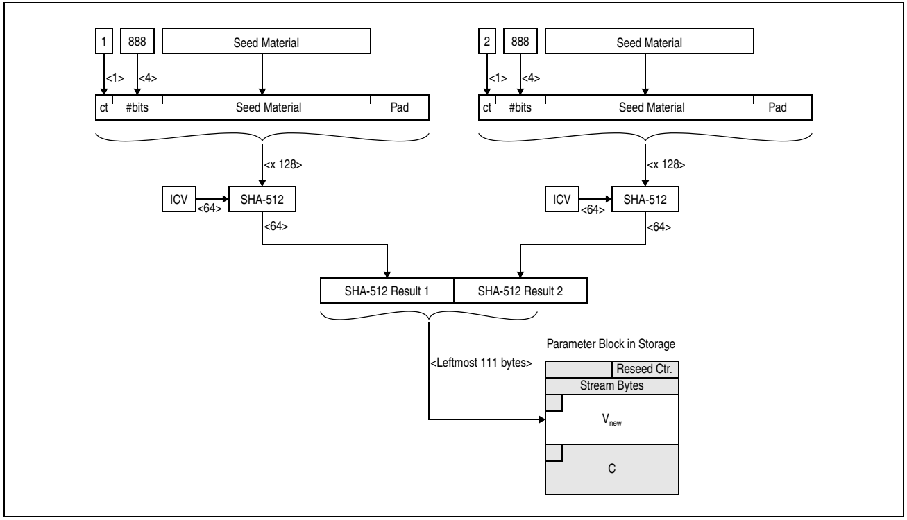
Figure 7-301. PPNO-SHA-512-DRNG Seed Operation's Formation of New Value ( V_{new} ) (Part 1 of 2)
