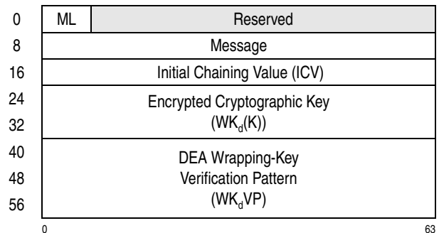
Figure 7-270. Parameter Block for PCC-Compute-Last-Block-CMAC-Using-Encrypted-TDEA-128
