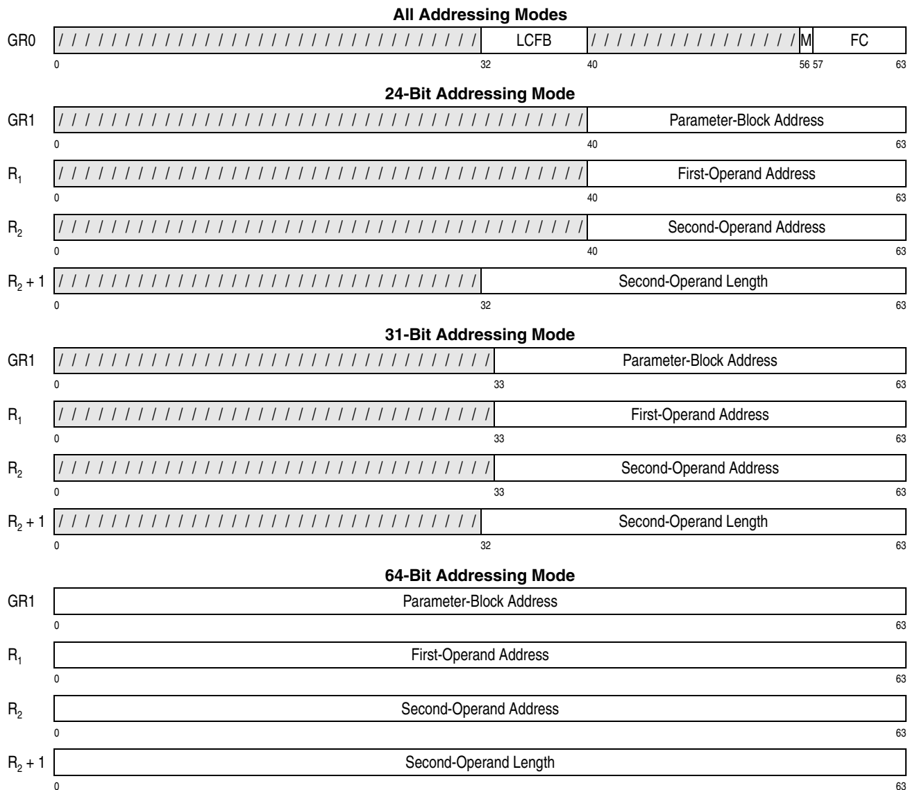
Figure 7-76. General Register Assignment for KMF
