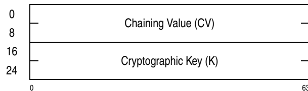
Figure 7-95. Parameter Block for KMF-AES-128
