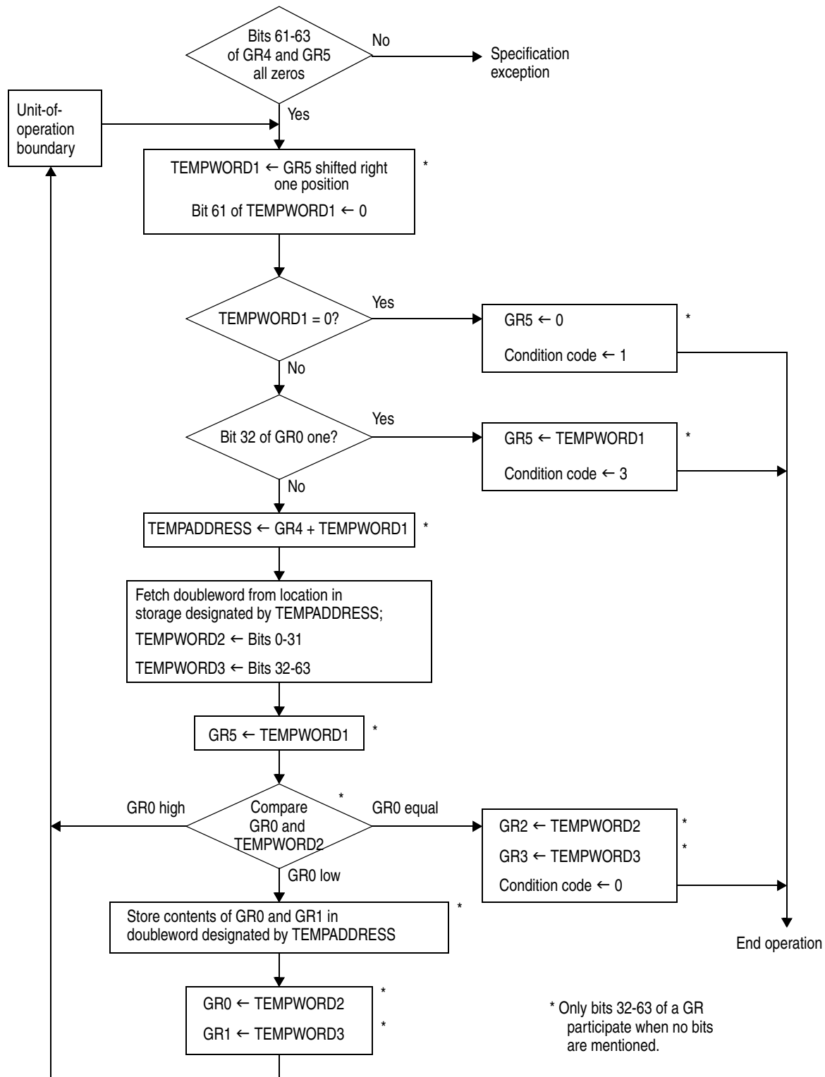
Figure 7-314. Execution of UPDATE TREE in the 24-Bit or 31-Bit Addressing Mode
