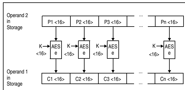
Figure 7-29. KM-AES Encipher Operation Using 128-Bit Key
