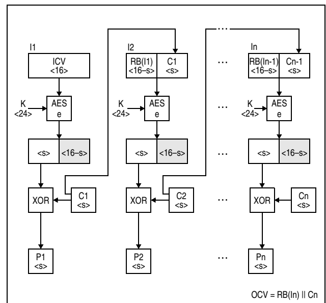
Figure 7-102. KMF-AES-192 Decipher Operation
