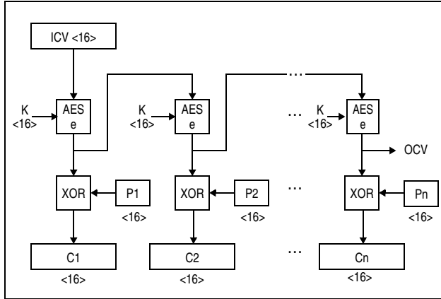
Figure 7-163. KMO-AES-128 Encipher Operation
