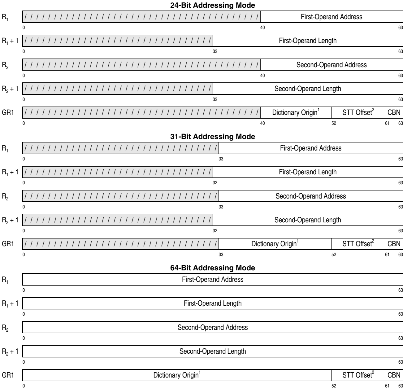
Figure 7-183. Register Contents for COMPRESSION CALL (Part 1 of 2)
