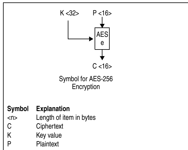
Figure 7-225. Symbols for AES-256 Encryption
