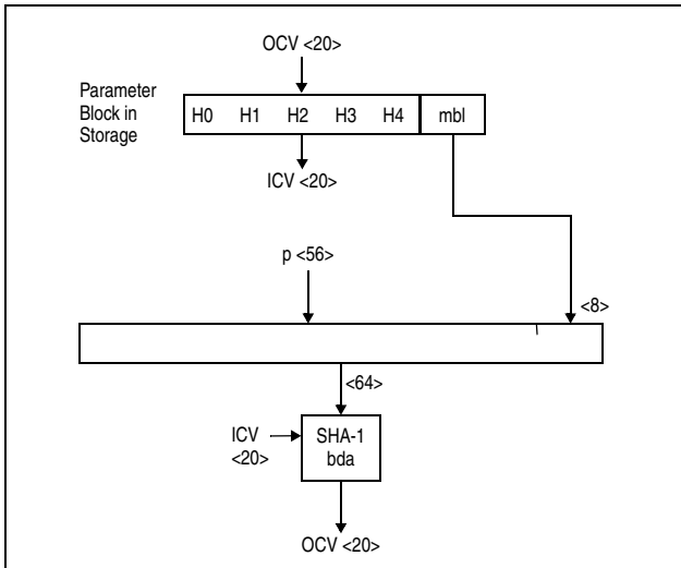
Figure 7-205. KLMD-SHA-1 Empty Block ( L = 0 )
