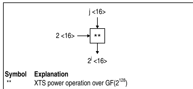
Figure 7-260. Symbol For XTS Power Operation Over GF(2^{128})
