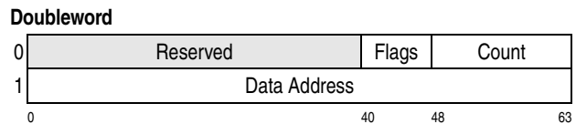
Figure 15-28. Modified-Indirect-Data-Address Word (MIDAW)
