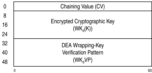
Figure 7-92. Parameter Block for KMF-Encrypted-TDEA-192
