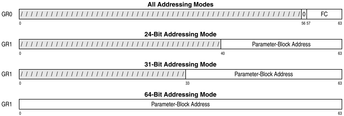
Figure 7-257. General Register Assignment for PCC
