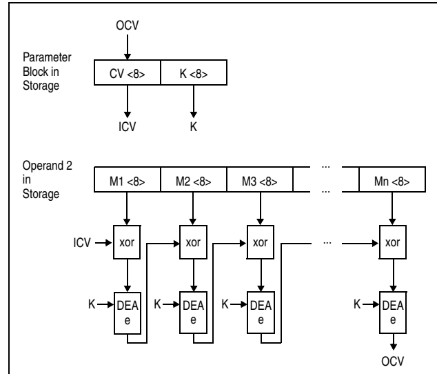
Figure 7-229. MAC Computation Using 64-bit DEA Key
