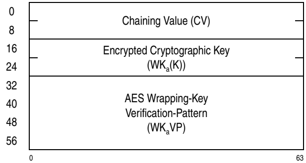
Figure 7-162. Parameter Block for KMO-Encrypted-AES-128
