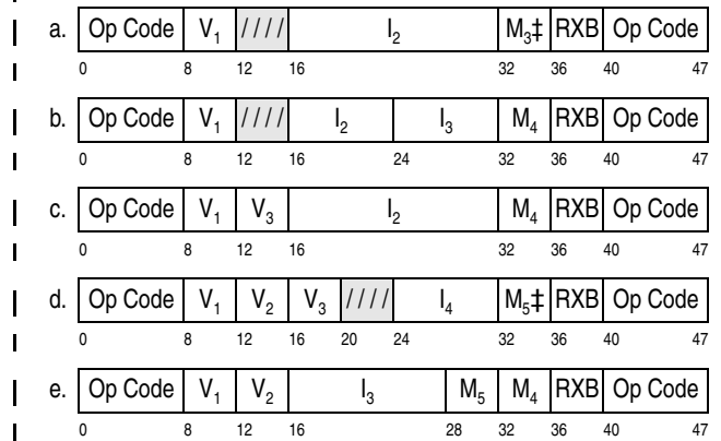
Figure 5-1. Basic Instruction Formats (Part 4 of 5)
