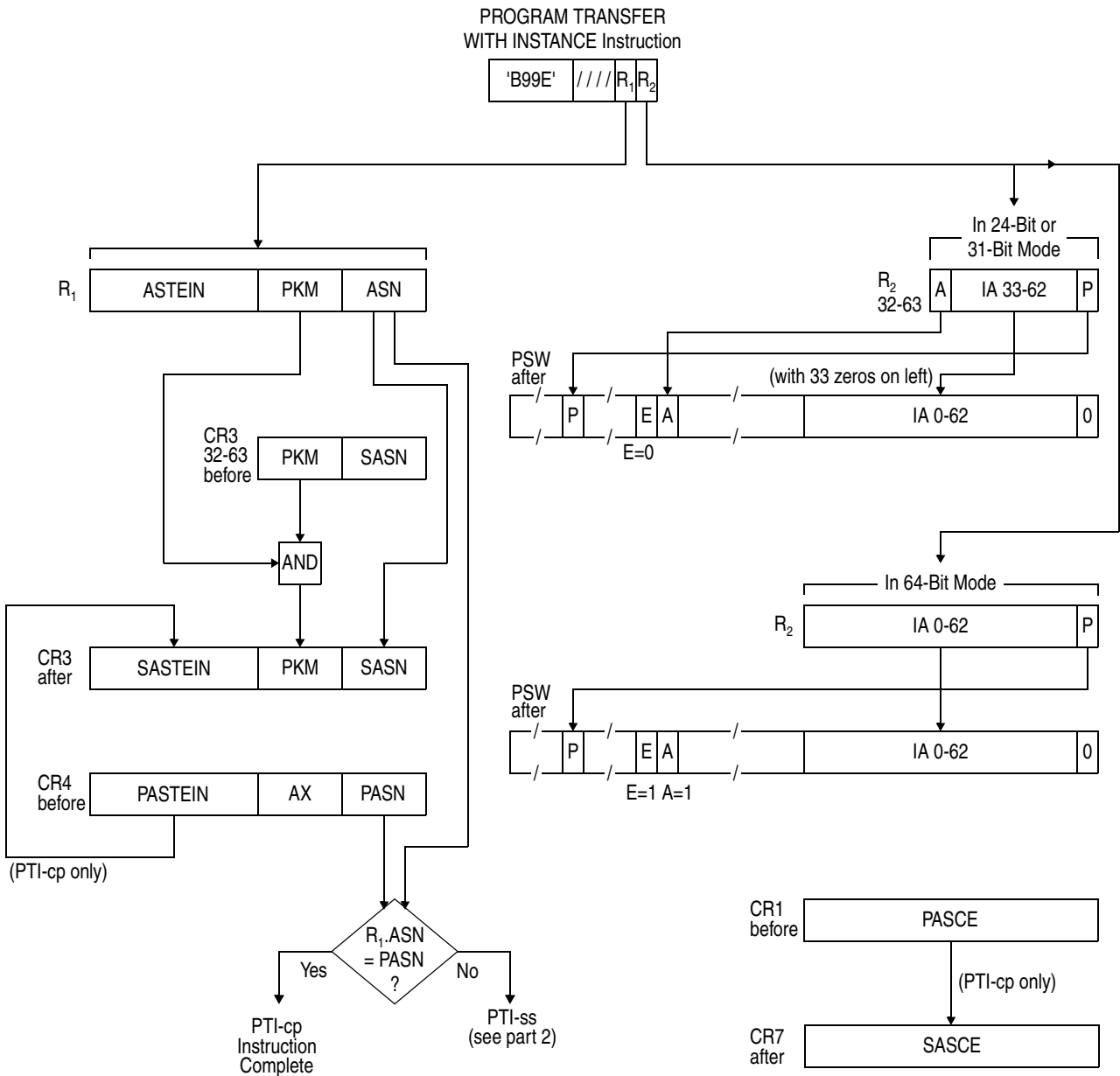
Figure 10-68. Execution of PROGRAM TRANSFER WITH INSTANCE (Part 1 of 2).
