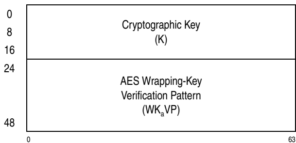
Figure 10-45. Parameter Block for PCKMO-Encrypt-AES-192-Key
