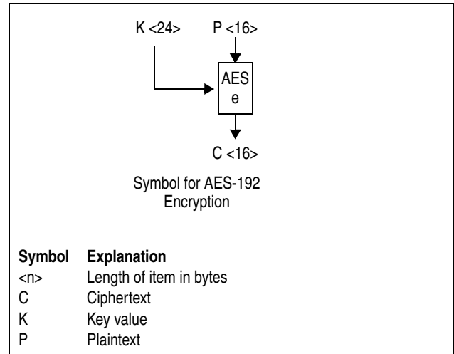
Figure 7-146. Symbols for AES-192 Encryption
