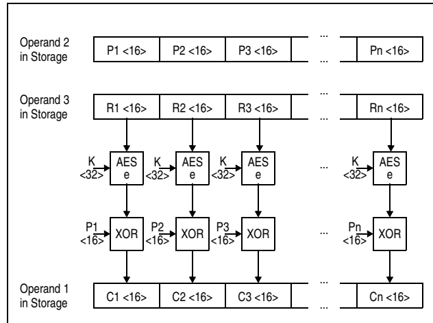
Figure 7-138. KMCTR AES Encipher Operation Using 256-Bit Key
