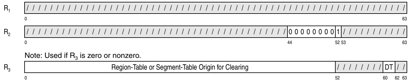
Figure 10-16. Register Contents for INVALIDATE DAT TABLE ENTRY Clearing-by-ASCE Operation (Bit 52 of GR R2 Is One)
