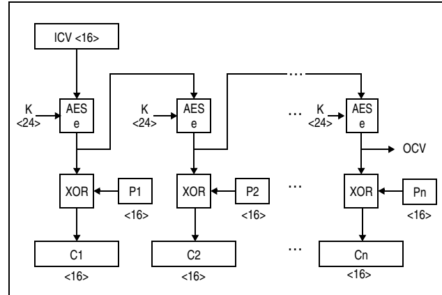
Figure 7-167. KMO-AES-192 Encipher Operation
