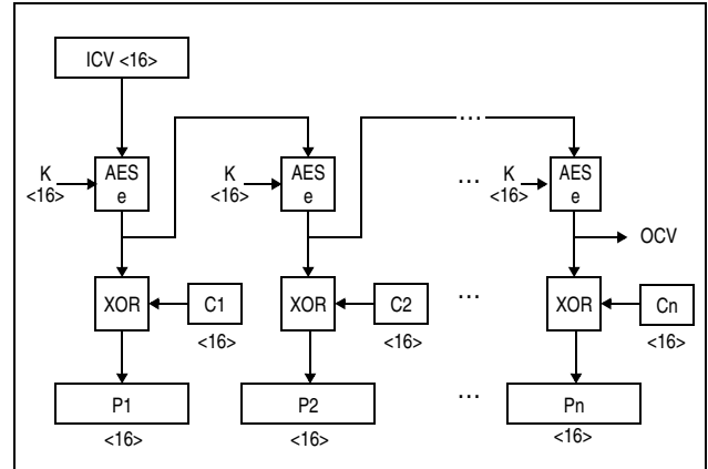
Figure 7-164. KMO-AES-128 Decipher Operation
