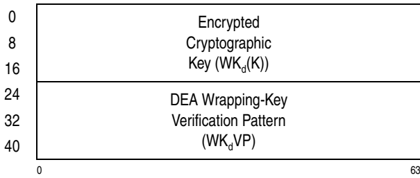
Figure 7-125. Parameter Block for KMCTR-Encrypted-TDEA-192
