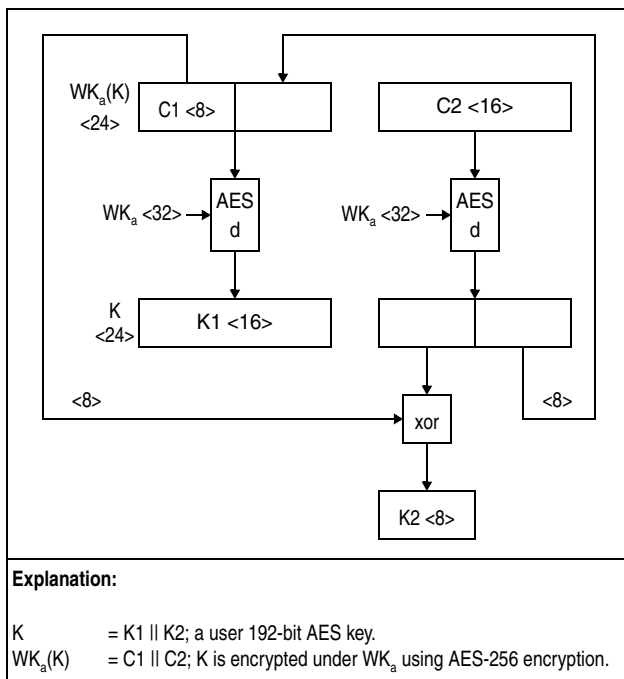
Figure 7-325. Decryption of 192-Bit AES Key Using WK_a
