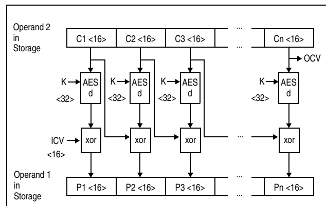
Figure 7-71. KMC AES Decipher Operation Using 256-Bit Key
