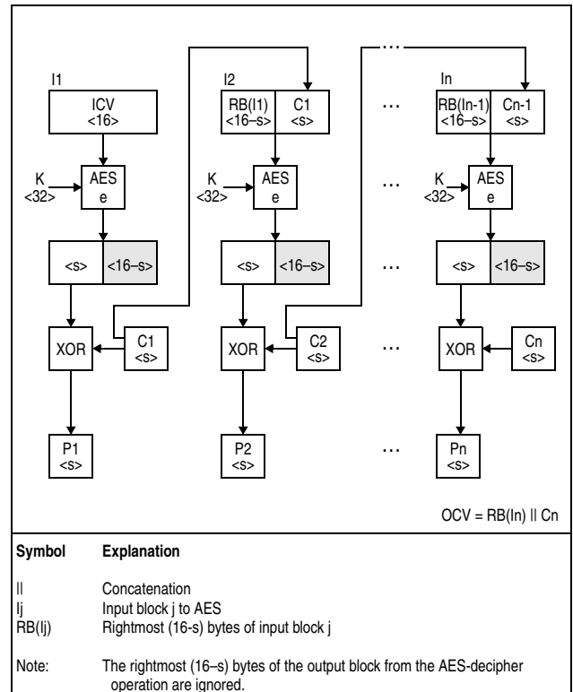
Figure 7-106. KMF-AES-256 Decipher Operation
