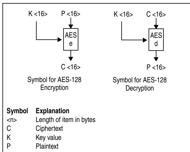
Figure 7-262. Symbols for AES-128 Encryption and Decryption
