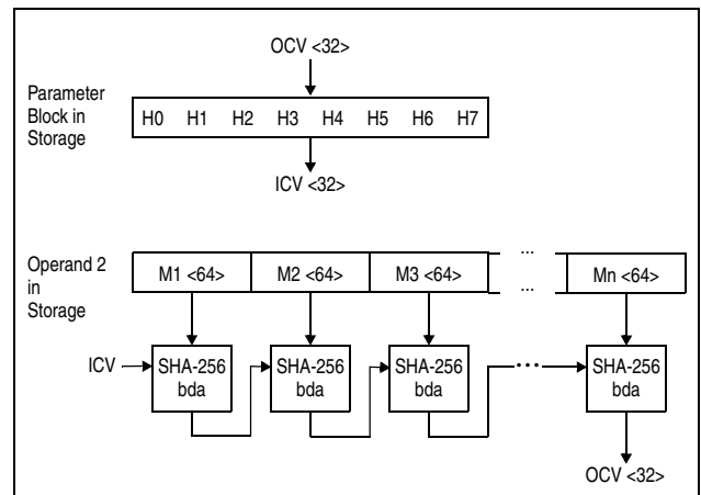
Figure 7-197. KIMD-SHA-256
