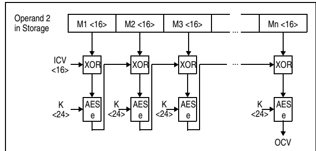
Figure 7-241. KMAC-AES-192
