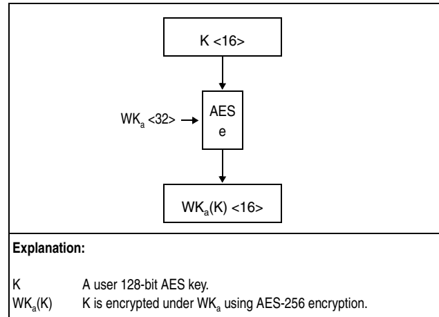
Figure 7-322. Encryption of 128-Bit AES Key Using WK_a
