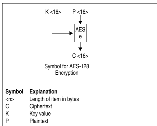
Figure 7-223. Symbols for AES-128 Encryption
