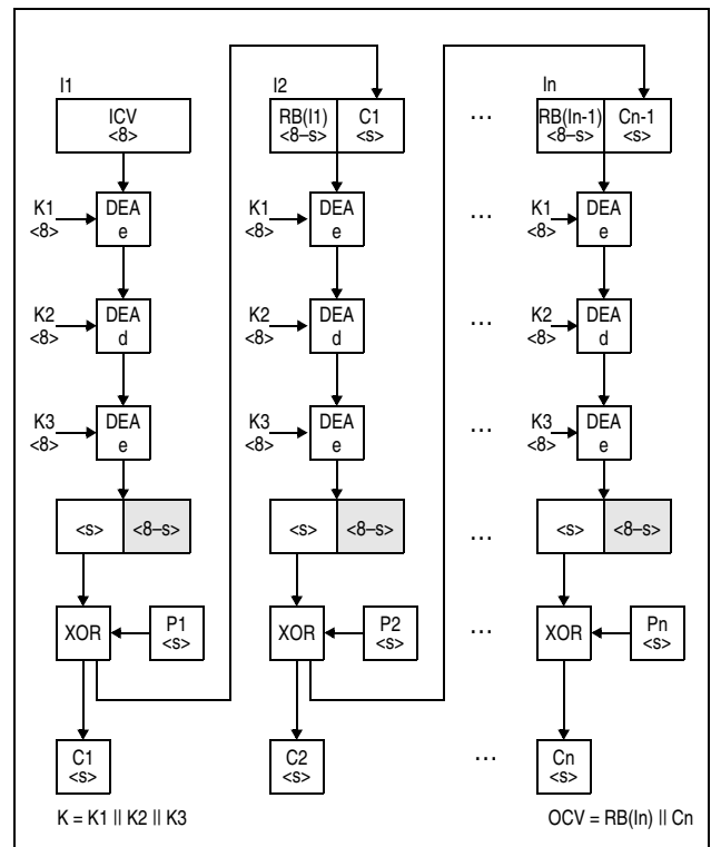
Figure 7-93. KMF-TDEA-192 Encipher Operation
