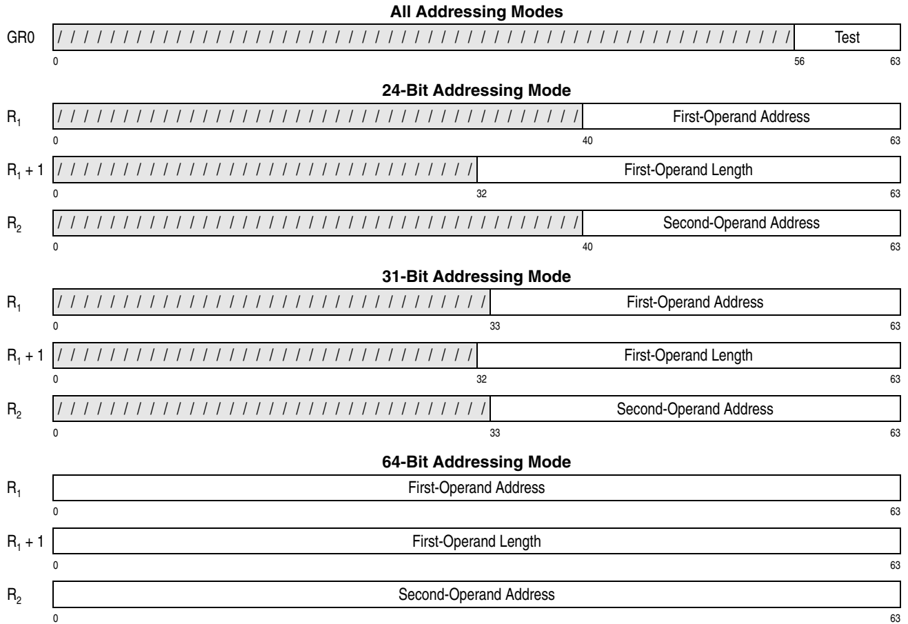
Figure 7-312. Register Contents for TRANSLATE EXTENDED
