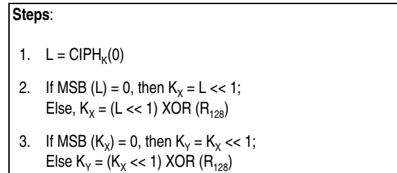
Figure 7-280. Subkey Generation Algorithm
