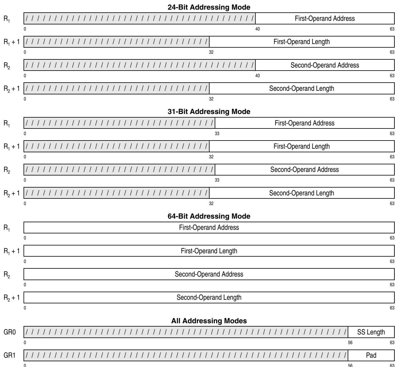
Figure 7-182. Register Contents and Second-Operand Address for COMPARE UNTIL SUBSTRING EQUAL
