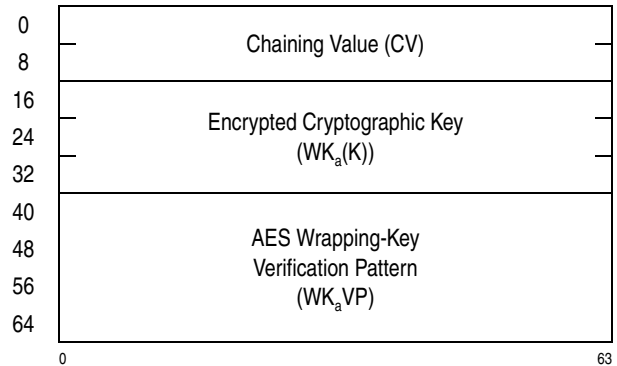
Figure 7-100. Parameter Block for KMF-Encrypted-AES-192
