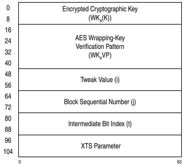
Figure 7-285. Parameter Block for PCC-Compute-XTS-Parameter-Using-Encrypted-AES-128
