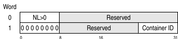
Figure 10-83. Container-Type Topology-List Entry
